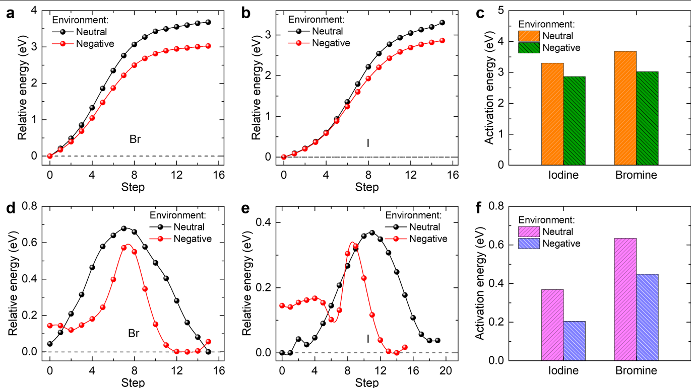
Extended Data Fig. 10 | Activation energy for halide migration. a–c , Energy profiles for the extra-lattice migration of a , bromine and b , iodine in a neutral uncharged or negatively charged environment, and c , corresponding
