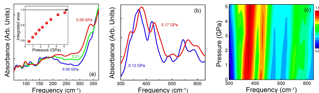
Figure 2. (a) Synchrotron-based far infrared spectrum of \text{Na}_9[\text{Ho}(\text{W}_5\text{O}_{18})_2] \cdot 35\text{H}_2\text{O} as a function of pressure in the 55\text{--}375\text{ cm}^{-1} region. Both intramolecular and intermolecular features are observed. Inset: Integrated area under the curve in the 220\text{--}310\text{ cm}^{-1} frequency window. The latter corresponds to the transparency window and was therefore used as the integration range. (b) Close-up view of the far infrared response of \text{Na}_9[\text{Ho}(\text{W}_5\text{O}_{18})_2] \cdot 35\text{H}_2\text{O} between 300 and 625\text{ cm}^{-1} . (c) The same data as in panel (b) shown as a contour plot. Spectra at 12 different pressures were used to create the contour plot.
