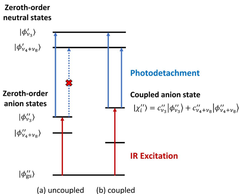
Figure 5. Schematic energy level diagram showing how additional photodetachment transitions arise due to anharmonic coupling of the v_3 mode with other vibrational levels. Anion and neutral zeroth-order states for the uncoupled case are shown on the left (a) and the excited anharmonically coupled eigenstate in the anion is shown on the right (b). IR excitation is shown by red arrows and detachment transitions are shown by blue arrows. The dashed arrow indicates a non-FC allowed transition. Note that only two zeroth-order states ( v_3 and v_4 + v_8 ) with the largest contributions to the coupled anion state are shown for clarity. Anharmonic coupling within the neutral is also neglected in this scheme and neutral zeroth-order states are shown instead for both cases.
