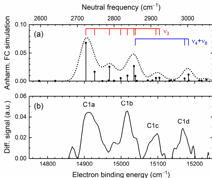
Figure 7. (a) Black stick spectrum shows the anharmonic Franck-Condon simulation for vinoxide excited via the \nu_3 fundamental in the eBE region near the expected 3_1^1 transition, calculated according to eq 5 in which anharmonic coupling for both the anion and neutral \nu_3 modes is included. Dotted line shows a convolution of the stick spectrum, scaled by an arbitrary scaling factor and using an eKE-dependent linewidth as described in Section S1.3. Colored combs indicate transitions that can nominally be assigned to the \nu_3 (red) and \nu_4 + \nu_8 (blue) anion zeroth-order states. Neutral frequencies shown at the top are related to the eBE by a shift of -EA + \nu_{3,\text{anion}} = -12181 \text{ cm}^{-1} , where the electron affinity is EA = 14721 \text{ cm}^{-1} and the anion frequency is estimated as \nu_{3,\text{anion}} = 2540 \text{ cm}^{-1} . (b) Experimental difference spectrum near the expected 3_1^1 transition based on the corresponding high-resolution scan from Figure 4b, which was measured at a photon energy of 15290 \text{ cm}^{-1} .
