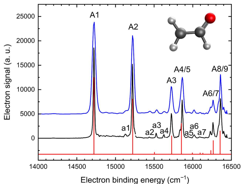
Figure 2. Top trace (blue curve): Overview photoelectron spectrum of the vinoxide anion taken at a detachment photon energy of 16446\text{ cm}^{-1} without IR excitation. Center trace (black curves): Corresponding high-resolution spectra taken at several lower photon energies and scaled to reflect the intensities in the overview spectrum. Bottom trace (red curve): Harmonic Franck-Condon simulation for detachment from the vibrational ground state of the anion (see Section 3.2 for details).
