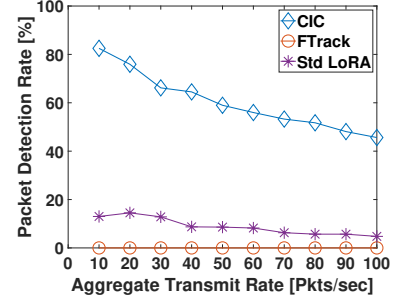
Fig 35: Packet Detection : D4 (Outdoor, SubNoise SNR, NLoS)
