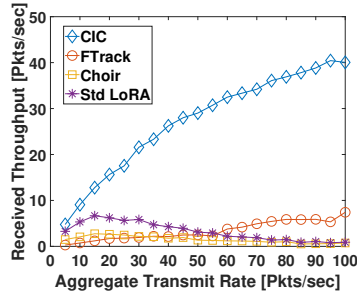
Fig 30: Network Capacity for D3 (Low SNR, NLoS)
