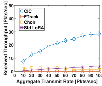
Fig 31: Network Capacity for D4 (Outdoor, SubNoise SNR, NLoS)
