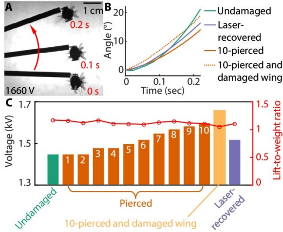
Fig. 5. Robot liftoff experiments under DEA and wing damage. (A) A liftoff demonstration performed by the same robot as in Fig. 4A. (B) Tracked beam angle during robot liftoff demonstrations. These liftoff experiments correspond to the static flapping-wing conditions in Fig. 4B. (C) Measured robot lift-to-weight-ratio at different damage conditions and driving voltages. Under different DEA and wing damage conditions, the robot net lift force remained higher than the robot weight.
