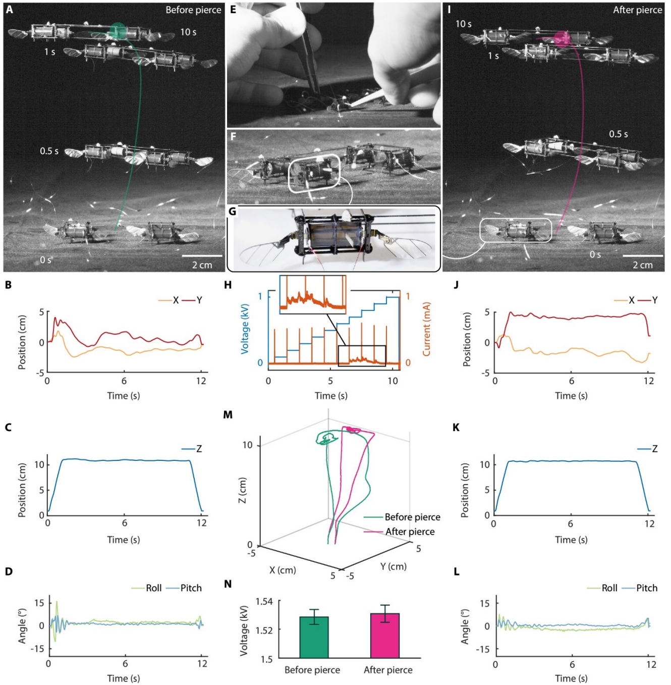
Fig. 6. Flight comparison of robots driven by undamaged and one-pierced DEAs. (A) A composite image that shows a twelve-second flight performed by an undamaged robot. (B-D) Robot x, y, and z positions and attitudes that correspond to the flight in (A). (E) A fiberglass needle pierced through a DEA. (F-H) The damaged DEA used self-clearing to isolate the defect. (I) A composite image that shows a twelve-second flight performed by the damaged robot. (J-L) Robot x, y, and z positions and attitudes that correspond to the flight in (I). (M) Comparison of flight trajectories between the damaged and the undamaged robot. (N) Comparison of average DEA operating voltages during the two hovering flights.
