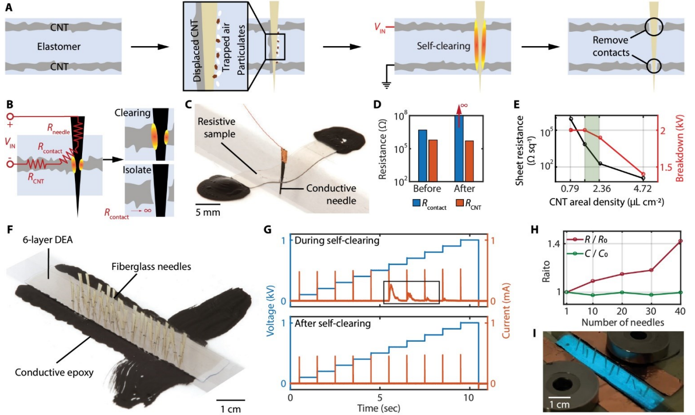
Fig. 2. Self-clearing of piercing damage in CNT electrodes. (A) Illustration of defect isolation through self-clearing. (B-C) Illustration (B) and experiment (C) of defect isolation in a resistive sample. (D) Contact ( R_{\text{contact}} ) and bulk CNT ( R_{\text{CNT}} ) resistances before and after self-clearing. (E) Electrode sheet resistance and dielectric strength as functions of CNT areal density. (F) An unrolled DEA was pierced by 40 fiberglass needles. (G) Applied voltage and measured current during and after self-clearing. The boxed region corresponds to thermal degradation of defects. (H) Change of DEA resistance and capacitance as functions of puncture counts. (I) Piercing test of an electroluminescent DEA showed that the bulk electrode connectivity was unaffected.
