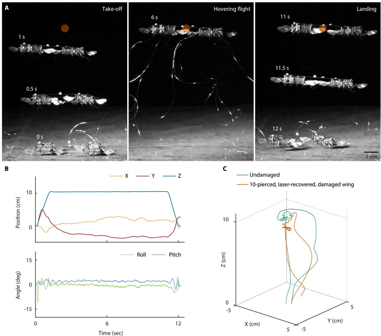
Fig. 7. Flight performance of a severely damaged soft-actuated aerial robot. (A) A twelve-second hovering flight performed by the severely damaged robot shown in Fig. 1B. One DEA was pierced by ten needles, the other DEA suffered an unclearable breakdown, and one robot wing lost 20% of its area. In this flight, the robot showed a one-second ascent (left), a ten-second hover (center), and a one-second descent (right). (B) Tracked robot positions and attitudes corresponding to the flight in (A). (C) Flight trajectory comparison of the two robots with or without damage.
