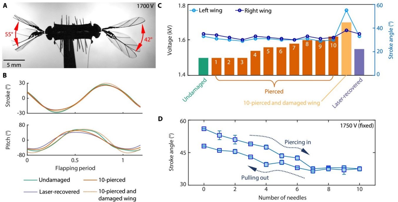
Fig. 4. Characterization of DEA damage resilience in static flapping-wing experiments. (A) A composite image of the robot flapping-wing kinematics. The DEA was pierced by ten needles and the left wing lost 20% area. (B) Robots with differently damaged actuators and wings could produce wing stroke and pitch motions that correspond to liftoff conditions. (C) Robot wing stroke amplitude at different damage conditions and driving voltages. Under DEA piercing damage, unclearable breakdowns, and wing damage labelled along the x-axis, the robot maintained similar wing stroke motion when the driving voltage was increased. These flapping kinematics conditions correspond to the liftoff conditions. (D) Degradation and recovery of robot stroke amplitude when needles were sequentially put in and then removed from the DEA. The error bars indicate the measured left- and right-wing stroke angles.
