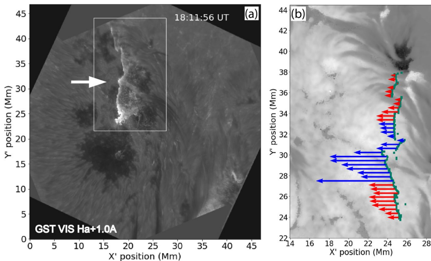
Fig. 16 Fine structure of a solar flare ribbon revealed by the 1.6 m GST in BBSO. a The VIS H\alpha+1.0 \text{ \AA} image shows the ribbon of the 2015-06-22T18:23 flare in NOAA AR 12371 with a light bridge indicated by the white arrow. b A zoomed-in view of the image shows the enhanced ribbon speed around the light bridge (blue arrows) and the ribbon front (green line) approximately parallel to the PIL. The enhanced speed ranges between 10 and 20 km/s (Courtesy of B. Cannon et al. 2022). A supplementary movie is available in Jing et al. (2016)
