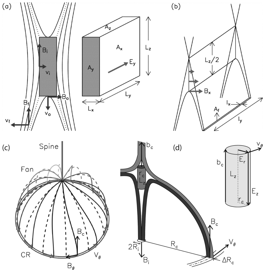
Fig. 4 Parameters used for formulating magnetic reconnection in PRF ( a, b ) and CRF ( c, d ). a An arcade system for 2D X-point inside the current layer (shaded area) and the separatrix (dotted lines). b The relationship between the coronal current layer and the flare ribbons. (Source: Lee et al. 2006). c A spine-fan system with (solid) and without (dashed) a torsional perturbation. d Layers of the fan fields connecting from the CR to the outer spine (light shade) and to the inner spine (dark shade) along with the current tube located around the 3D null point
