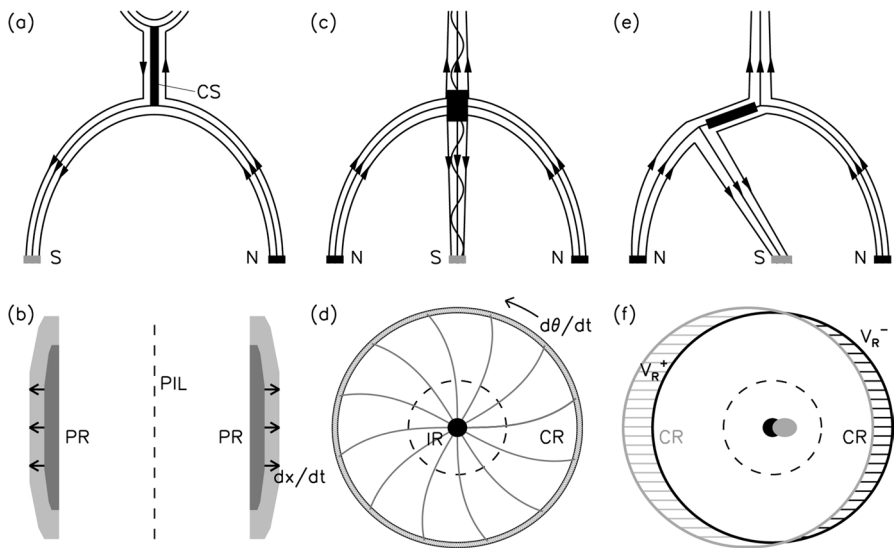
Fig. 5 Schematic illustration of the three types of reconnection: 2D X-point ( a , b ), torsional ( c , d ), and spine-fan ( e , f ) reconnection. Upper panels show the side views of the magnetic configurations in which N and S refer to the magnetic polarity in the footpoints and the filled arrows, the polarity of the coronal fields. The black regions in the corona represent the nonideal region. Lower panels show the top-down views in which three types of ribbons, PR, CR, and IR are denoted together with their motions in the translational, rotational, and vibrational degrees of freedom. Dashed lines are PILs
