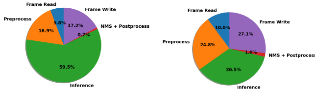
Fig. 12: Time profile breakdowns of the TensorRT anonymization pipeline with model input resolution of 960 \times 960 on T4 GPU with batch size of 1 (left) and 608 \times 608 on A100 GPU with batch size of 8 (right). Both profiles use FP16 precision.
