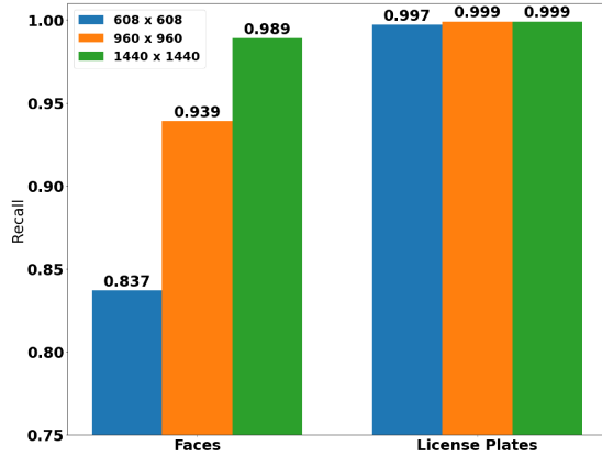
Fig. 8: Validation recall of face and license plates with cross section areas larger than the visible pixel area threshold.
