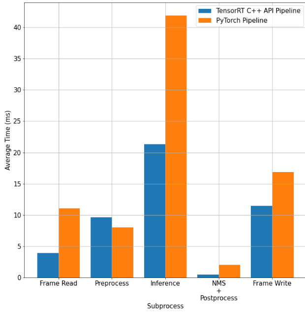
Fig. 11: Average time by subprocess of the PyTorch and TensorRT anonymization pipelines configured with the 960 \times 960 input resolution model, batch size of 1, and FP32 precision.
