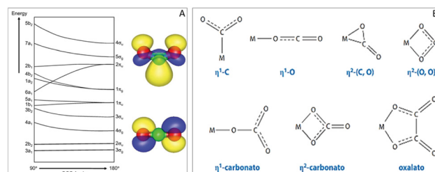
Fig. 8 (A) Walsh diagram of \text{CO}_2 , with illustrations of the highest occupied molecular orbitals of the anion (top) and the neutral (bottom). (B) Structural motifs of metal- \text{CO}_2 interactions. Reprinted from ref. 43 and 44 with permission. Copyright 2014 Abingdon: Taylor & Francis and 2018 Annual Reviews.
