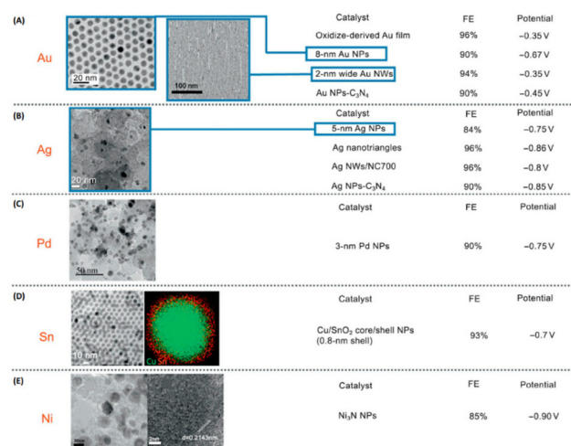
Fig. 15 Summary of some representative nanocatalysts based on Au (A), Ag (B), Pd (C), Sn (D) and Ni (E) for electrochemical CO 2 RR to CO. All potentials are vs. RHE. NP denotes nanoparticle and FE is the reported faradaic efficiency. Adapted from ref. 93 with permission. Copyright 2019 Cell Press.
