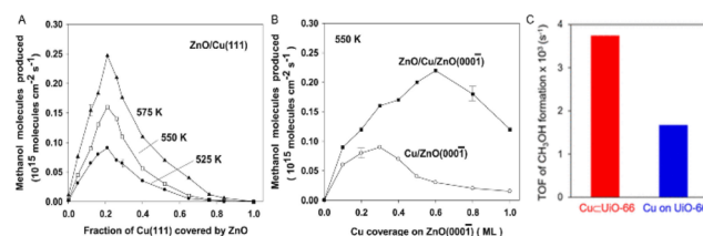
Fig. 12 (A, B) \text{CO}_2 conversion to methanol. (C) Initial TOFs of methanol formation over \text{Cu}/\text{UiO-66} and Cu on \text{UiO-66} . The reaction rates were measured after 1 h. Reaction conditions: 7 sccm of \text{CO}_2 , 21 sccm of \text{H}_2 , 10 bar, and 175 °C. Adapted from ref. 66 and 70 with permission. Copyright 2017 American Association for the Advancement of Science and 2016 American Chemical Society.
