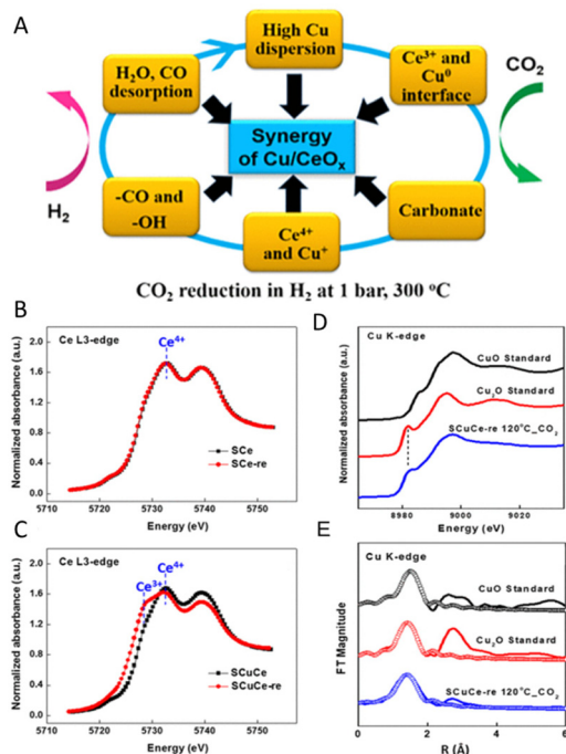
Fig. 11 (A) Schematic illustration of synergy of \text{Cu}/\text{CeO}_x for \text{CO}_2 hydrogenation. (B–E) XAS spectra of Cu and Ce oxidation state change during reaction (note that SCe = SBA-supported \text{CeO}_2 and SCuCe = SBA-supported Cu– \text{CeO}_2 ). Adapted from ref. 61 with permission. Copyright 2018 American Chemical Society.
