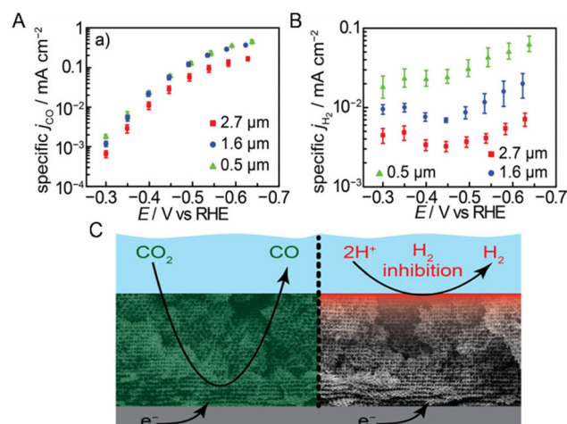
Fig. 18 Specific activity for CO (A) and H 2 (B) with different thickness of Au-IO: 0.5 \mu m (green triangles), 1.6 \mu m (blue circles), and 2.7 \mu m (red squares). The samples were evaluated in CO 2 -saturated 0.1 M KHCO 3 electrolyte, pH 6.7. Error bars represent standard deviations of three independently synthesized Au-IO samples for each thickness. (C) Scheme represents the mesostructure-induced pH gradient during CO 2 RR. Adapted from ref. 153 with permission. Copyright 2015 American Chemical Society.
