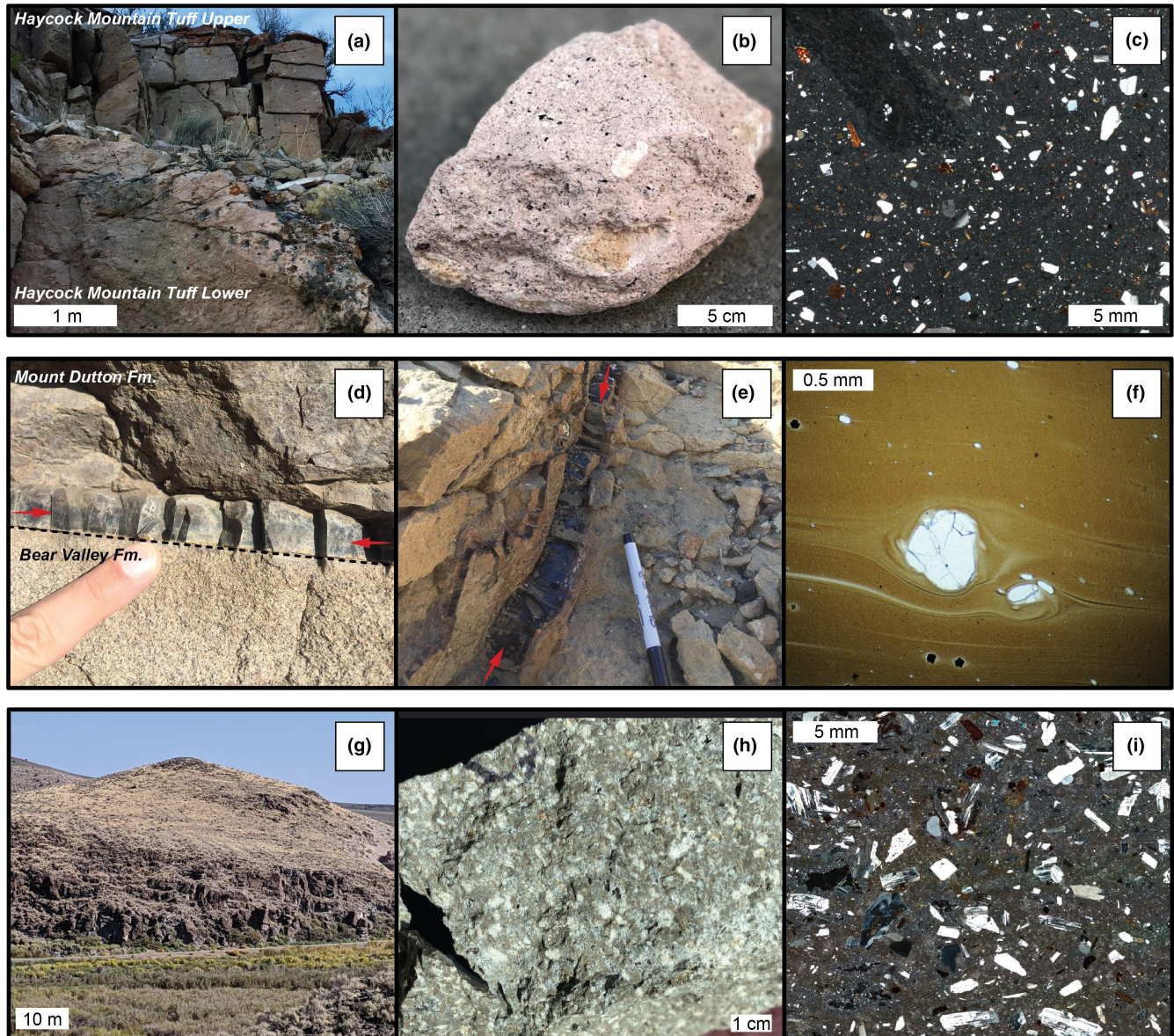
FIGURE 2 (a) Outcrop of Haycock Mountain Tuff showing the lower massive and upper densely welded units. (b) Hand sample of lower Haycock Mountain Tuff showing pumice fragments (white and brown, centre) and prominent biotite phenocrysts. (c) Portion of a thin section of the Haycock Mountain Tuff; cross-polarized light. (d) Pseudotachylyte vein (red arrows) between Bear Valley Formation sandstone and the Mount Dutton Formation. (e) Pseudotachylyte vein (red arrows) within the Bear Valley Formation sandstone. A ~2 mm thick chilled margin can be seen on the right side. (f) Pseudotachylyte and relict quartz in thin section; plane-polarized light. (g) Outcrop of undeformed Osiris Tuff. (h) Hand sample of Osiris Tuff showing feldspar dominating the phenocryst assemblage. (i) Portion of a thin section of the Osiris Tuff, cross-polarized light
