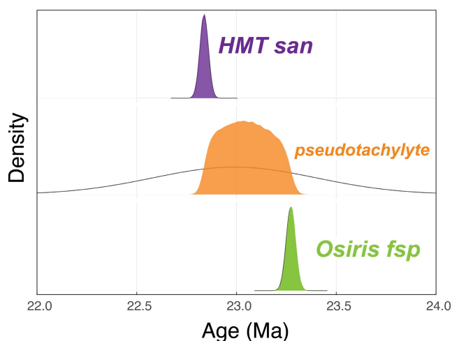
FIGURE 4 Summary of geochronology and Bayesian modelling results. The solid lines are the probability distribution functions of the ^{40}\text{Ar}/^{39}\text{Ar} date for each sample. The shaded regions are posterior density estimates of age from the Bayesian recalibration considering the relative order of events. The modelled age for the gravity slide pseudotachylyte is 23.05 \pm 0.22/–0.20 Ma (median \pm 95% credible interval)
