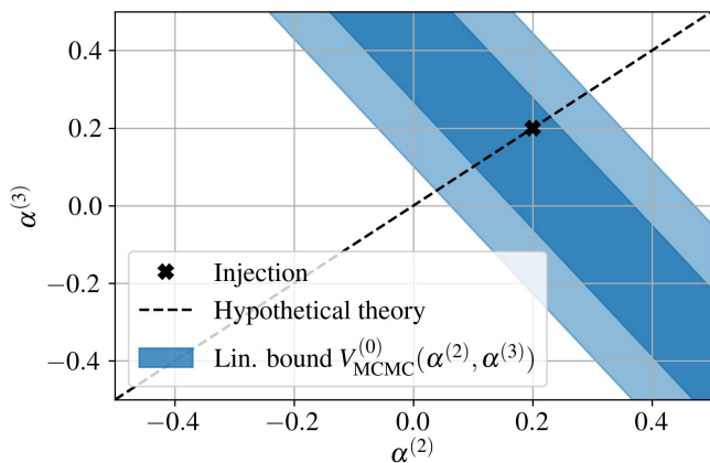
FIG. 7. Post-processing analysis using the posterior of V^{(0)} . Blue areas show the 1\sigma and 2\sigma confidence levels on the functional relation \alpha^{(3)}(\alpha^{(2)}, V^{(0)}) . The black dashed line indicates the linear relation assumed in the hypothetical theory. The black dot is the intersection of the maximum of the posterior with the theory-specific relation, while the cross is the injected value.
