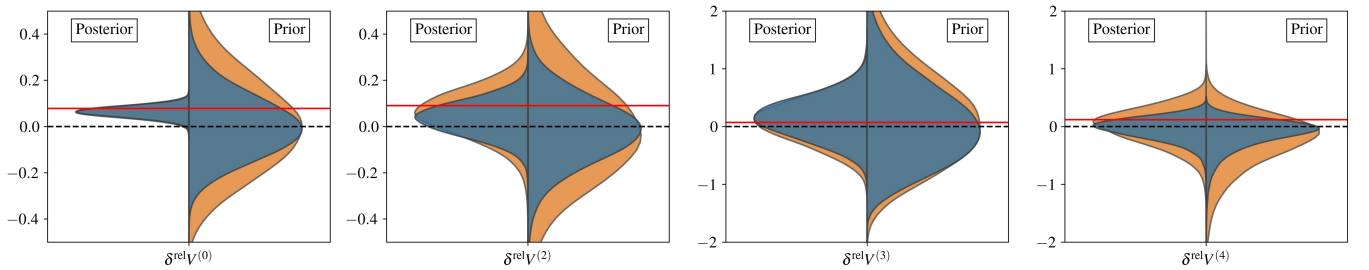
FIG. 5. Same MCMC results as in Fig. 4, but here we sample the relative errors of various derivatives of the effective potential \delta^{\text{rel}} V^{(n)} with respect to the tortoise coordinate evaluated at the maximum. The right side of each violin plot shows the sampling from the prior distribution of all \alpha^{(k)} simultaneously. The colors label the different \alpha^{(k)} prior ranges, \alpha_{P20}^{(k)} (blue) and \alpha_{P10}^{(k)} (orange). The left side of each violin plot shows the sampling from the posterior distributions, with colors labeling the prior assumptions. We mark the injections by horizontal red lines.
