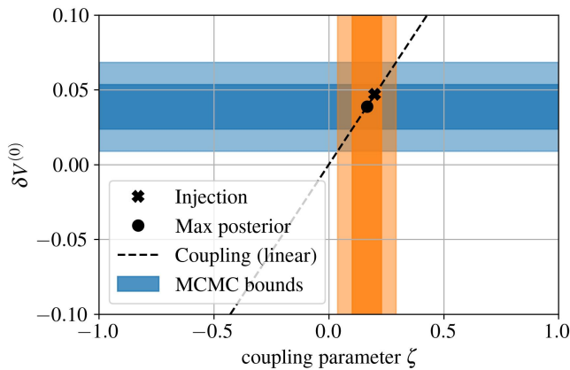
FIG. 6. Post-processing analysis using the posterior of V^{(0)} . Blue areas show the 1\sigma and 2\sigma confidence levels of the theory-agnostic analysis, while the orange areas label the corresponding bounds on the theory-specific parameter \zeta . The black dashed line indicates the linear scaling predicted by Eq. (9). The black dot shows the maximum of the posterior, and the cross is the injected value.
