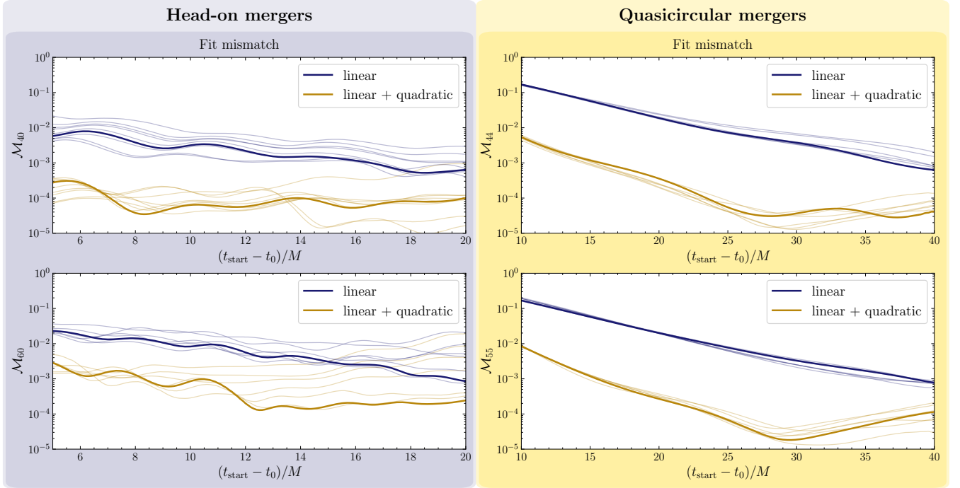
FIG. 5. The mismatch \mathcal{M}_{\ell m} between the fitted waveform and the actual waveform in the \ell m harmonic of the head-on (left column) and quasi-circular merger (right column) simulations. The blue curves corresponds to fits consisting containing only the linear modes identified in the waveform, while the gold curves include also the corresponding quadratic mode. The highlighted lines correspond to \gamma = 2 for the head-on mergers, and SXS:BBH:0305 (top) and SXS:BBH:0403 (bottom) for the quasicircular mergers. For each individual simulation, the model containing the quadratic mode always has smaller mismatch.
