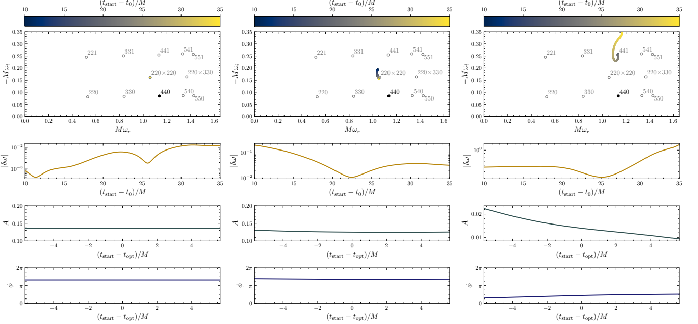
FIG. 7. Results for toy model A (left column), B (middle column) and C (right column).
