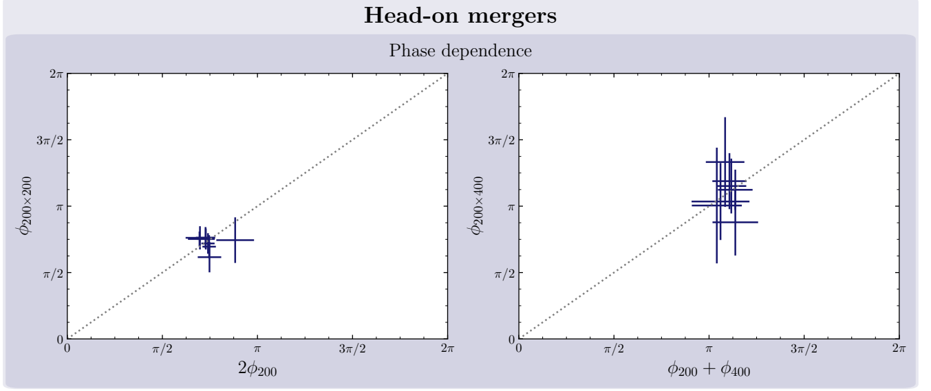
FIG. 4. The relationship between the phase of the second-order modes and that of the sourcing first-order modes for the head-on merger simulations, similar to the right column of Fig. 2. Different crosses correspond to simulations with different boosts \gamma , and the width and height of the crosses are the errors. The gray dotted line is the expected relationship.
