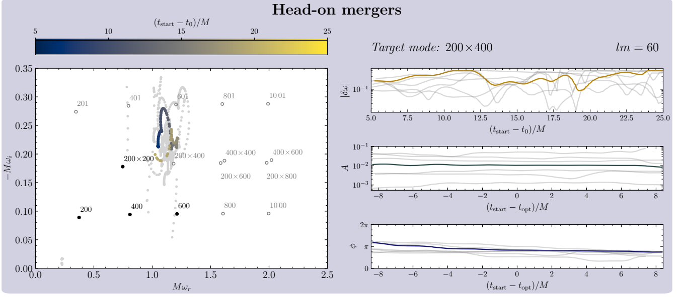
FIG. 6. Results for the 200 \times 400 mode search in the \ell m = 60 harmonic for head-on mergers (see Fig. 1). Free mode search (left); deviation of fitted frequency from expected second-order value (top right); amplitude (center right) and phase (bottom right) of the fitted mode around the starting time with lowest |\delta\omega| , with frequency fixed at the second-order value.
