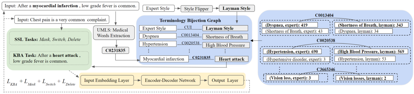
Figure 1: Multi-Task Self-Supervised Learning integrates KBA with Mask , Switch , Delete tasks. Four losses are optimized concurrently. The parameters of input embedding layer, encoder-decoder network and output layer are shared between pretraining and fine-tuning. On the right side, we demonstrate the construction of the Terminology Bijection Graph through edge refinement.
