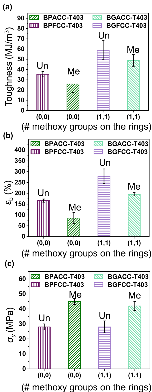
Figure 5. (a) Toughness, (b) \epsilon_b , and (c) \sigma_y as a function of the number of methoxy groups on the rings with the bridging-carbon substitution as bar labels.
