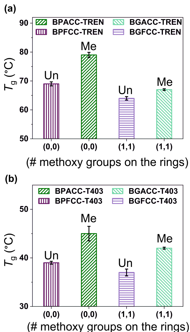
Figure 2. T_g as a function of the number of methoxy groups on the rings with the type of bridging-carbon substitution as bar labels for (a) TREN-based NIPU networks and (b) T403-based NIPU networks. Error bars indicate standard deviations of the measurements.
