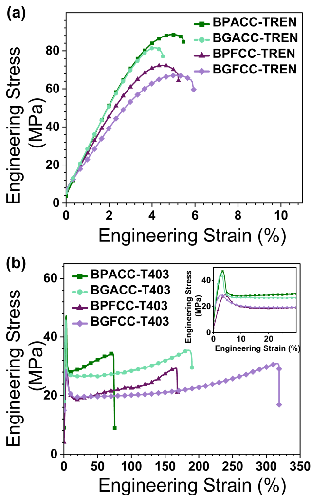
Figure 4. Representative engineering tensile stress versus engineering strain of (a) TREN-based NIPU networks and (b) T403-based NIPU networks obtained from uniaxial tensile testing using a load cell of 100 N and an extension rate of 10 mm/min at ~20 °C.
