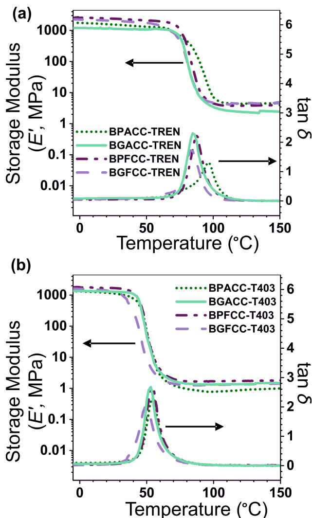
Figure 3. Storage modulus and \tan \delta as a function of temperature for (a) TREN-based and (b) T403-based NIPU networks. Data shown are from the second heating cycle of DMA experiments, in oscillatory film tension mode at a heating rate of 3 °C/min, strain amplitude of 0.3%, frequency of 0.1 Hz, and an axial force of 0.4 N.
