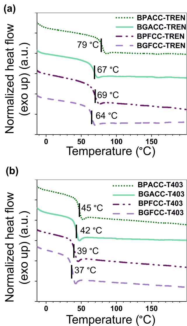
Figure 1. Representative DSC second heating traces of (a) TREN-based and (b) T403-based NIPU networks (10 °C/min, N 2 ). Curves are shifted vertically for clarity with T_g values marked on the respective curves. Each tick mark on the y-axis represents a 0.1 W/g increment.
