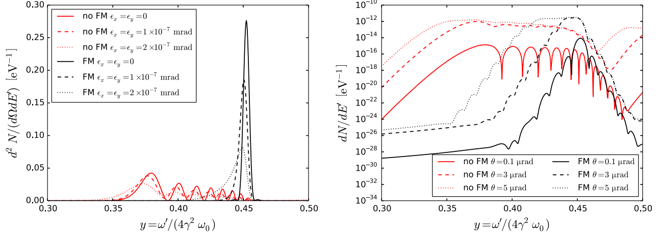
FIG. 2. Radiation spectrum for the nonlinear Compton scattering: uncompensated spectrum (no FM) is shown in red lines and optimally compensated (FM) in black. Left: Backscattered spectra ( d^2N/(d\Omega dE') ) for an electron beam with zero emittance (or for a single, on-axis particle) are shown in solid lines; \epsilon_x = \epsilon_y = 10^{-7} mrad emittance in dashed; and \epsilon_x = \epsilon_y = 2 \times 10^{-7} mrad emittance in dotted lines. Right: Spectra collected over a finite aperture, dN/dE' , for an electron beam with zero emittance (or for a single, on-axis particle) and: \theta = 0.1 \mu\text{rad} shown in solid lines; \theta = 3 \mu\text{rad} shown in solid lines; \theta = 5 \mu\text{rad} shown in solid lines. The solid red and black lines in both panels correspond to the same-colored lines in the top panel of Fig. 4 in Ref. [20] and the top panel of Fig. 2 in Ref. [21]. Spectra shown are for a linearly polarized 800-nm laser with pulse duration of 21 fs and a_0 = 1 on an Gaussian-distributed electron beam with mean energy of 51 GeV.
