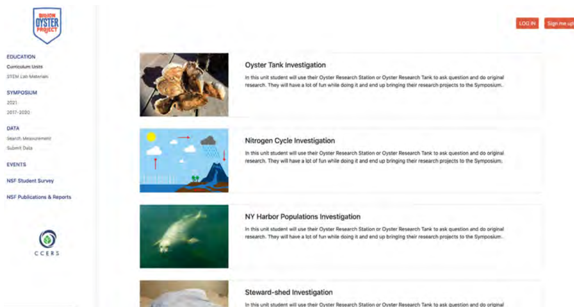
Figure 4. STEM Curriculum
