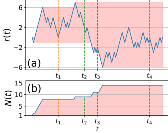
FIG. 1. (a) Space-time trajectory of a one-dimensional discrete random walk and (b) its corresponding span N(t) . At times t_1 , t_2 , t_3 , and t_4 (dashed lines), we are interested in the joint statistics of N(t_1) , N(t_2) , N(t_3) , and N(t_4) .
