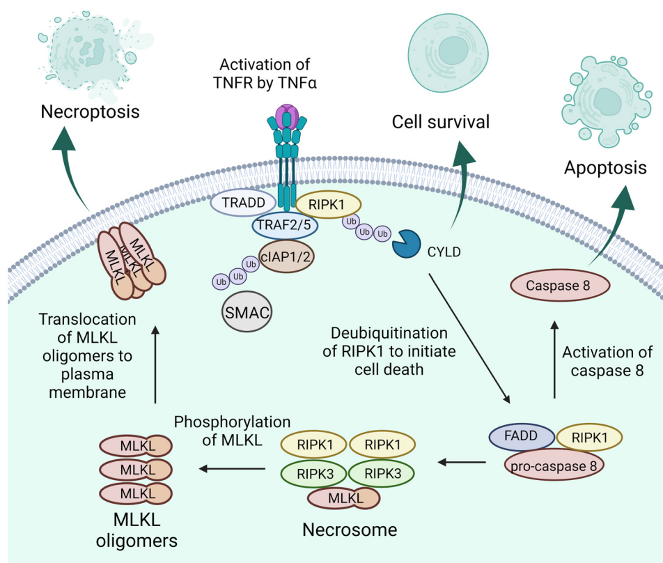
Fig. 1 Different cell fates following initiation of TNF \alpha signaling depend upon the ubiquitination of RIPK1 and activity of caspases. TNF receptor activation by binding to TNF \alpha causes recruitment of several adaptor proteins such as receptor interacting protein kinase 1 (RIPK1), TNF receptor type-1 associated death domain (TRADD), TNF receptor associated factor 2 (TRAF2), TNF receptor associated factor 5 (TRAF5) and cellular inhibitor of apoptosis protein 1 and 2 (cIAP1/2). cIAPs can cause ubiquitination of RIPK1 and initiate a cell survival signal. Cyldromatosis (CYLD) or second mitochondria-derived activator caspase (SMAC) can deubiquitinate RIPK1 and initiate a cell death signal. RIPK1 can recruit Fas associated via death domain (FADD) and procaspase 8 to initiate apoptosis or form a necrosome with receptor interacting protein kinase 3 (RIPK3) and mixed lineage kinase domain like pseudokinase (MLKL) in the absence of caspase 8 to initiate necroptosis. Phosphorylated MLKL oligomerizes and translocates to the plasma membrane leading to necroptosis-associated membrane permeabilization. Figure created with BioRender.com.
