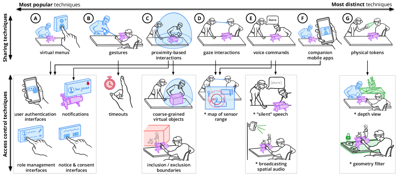
Figure 4: Evolution of AR sharing techniques into access control techniques. We illustrate the expert-elicited techniques for sharing AR content in HMD-based environments (mapped from most popular to most distinct, from left to right) and corresponding access control techniques that were added on to address threats. We indicate distinct techniques with (*). Virtual menus (A) were often paired with additional menus for user authentication, notifications, role management, and notice & consent. Gestures (B) were extended with timeouts, which limit the time period that AR devices accept gestural input. Proximity-based interactions (C) were extended through coarse-grained virtual objects (to maintain confidentiality of AR content while promoting awareness for other AR users) and inclusion/exclusion boundaries to define areas of the physical environment that can be captured. Gaze and voice commands (D, E) were combined with a virtual map of the sensor range to promote awareness of input hijacking attacks. For voice, experts also proposed silent speech to disclose less detail and broadcasting spatial audio, to promote awareness for bystanders while retaining some degree of confidentiality. Companion mobile apps (F) were paired with similar access control interfaces as virtual menus. Finally, distinct techniques involving physical tokens (G) led to distinct access control proposals for sharing depth views rather than RGB camera feeds and “locking” updates to AR devices’ spatial maps to prevent losing access to app content, in the event that marker-less tracking is disrupted.
