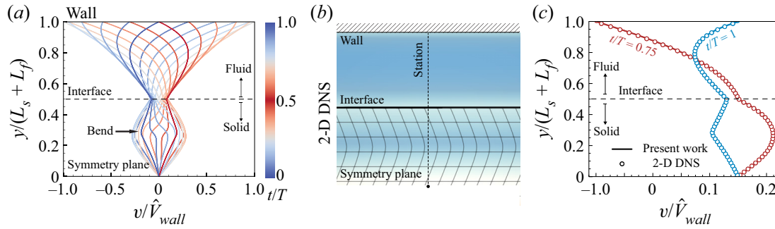
Figure 6. Comparison against simulations. (a) Non-dimensional velocity profiles in y , for a nonlinear Kelvin–Voigt solid. The system response is shown only in the upper half-plane. This system is characterized by Re = 2 , Er = 1 , \nu = 0.1 , c = c_3/c_1 = 4 , \delta_f = 0.4 , \delta_s = 0.126 , \lambda = 0.225 . Additional details can be found in supplementary material § 6. Colours indicate t/T . We also mark a high curvature bend in the profile with a black arrow. (b) We solve the above problem through 2-D DNS (Bhosale et al. 2021) with corresponding simulation parameters reported in supplementary material § 6. In this image, we mark the x -velocity field (orange/blue represent positive/negative velocity) and deformation contours within the solid, with the interface marked (black, thick solid) for visual clarity. Upon plotting the velocity profiles at the highlighted station (black, dashed) in the centre of the domain, we see good agreement with our results across all times as shown in (c). For the sake of clarity, we show profiles at only two different time instances. Here, numerical results are plotted with scatter points, whereas present results are plotted with a solid line.
