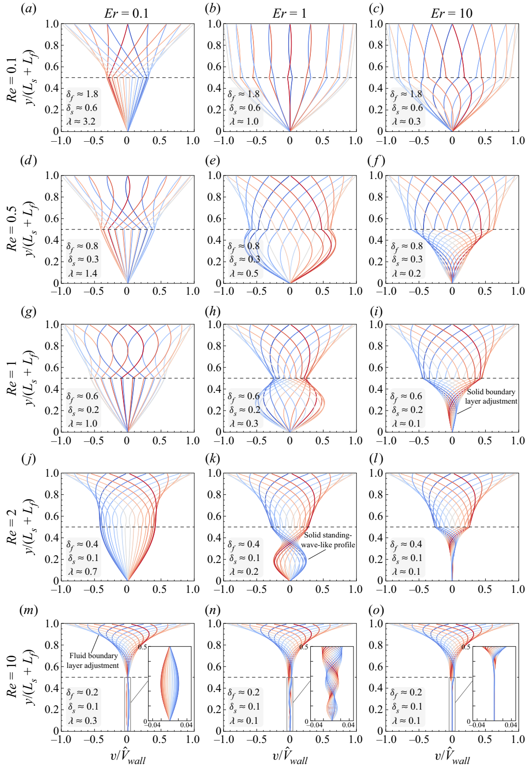
Figure 4. Dynamics with parametric variation. Non-dimensional velocity profiles in y for parametric changes in Re = \{0.1, 0.5, 1, 2, 10\} \times Er = \{0.1, 1, 10\} , with \nu = 0.1 , \rho = 1 . The system response is shown only for the upper half-plane, where we also mark the length scales \delta_f , \delta_s , \lambda . The black dashed lines indicate the solid–fluid interface. Colours represent t/T , with the same colour bar as in figure 2.
