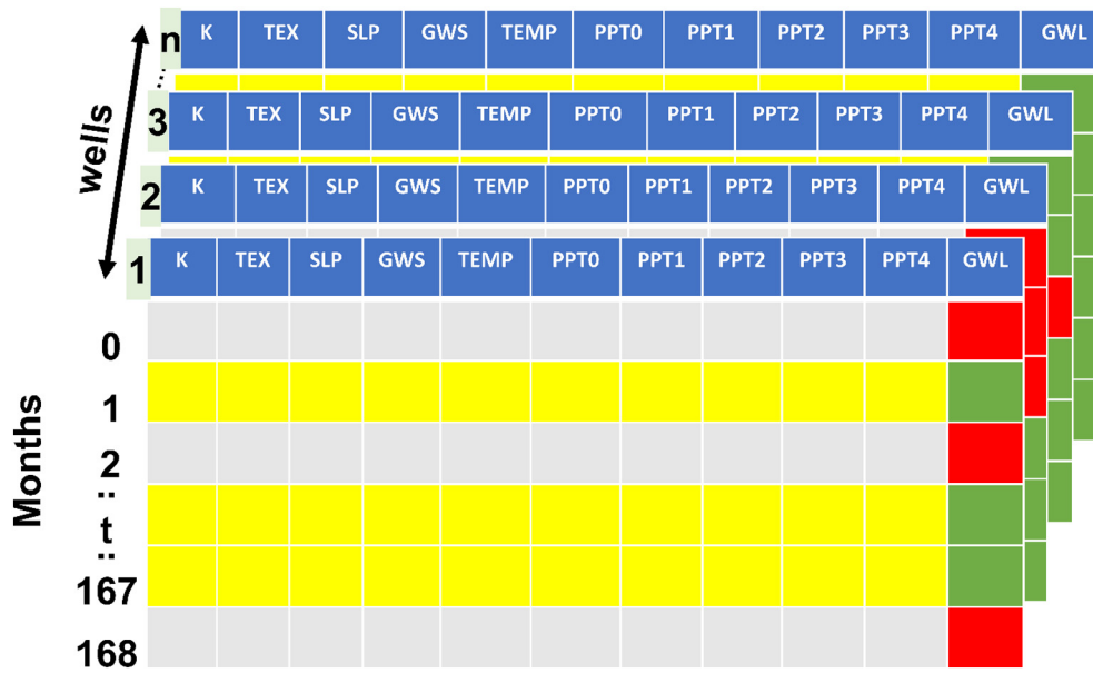
Fig. 3. Prepared input-output data patterns for Random Forest model. We compile data for the wells (numbered 1, 2, 3, ..., n ) separately for San Joaquin and Sacramento Valley for all 168 months covering our study period. Here n represents the number of wells in the respective region. Column GWL represents the response variable, while rest of the columns represent the input variables.
