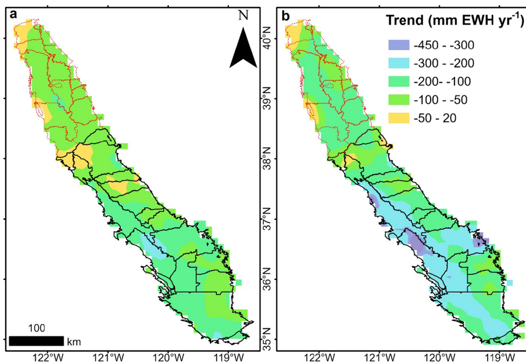
Fig. 9. Spatial variations in modeled groundwater storage trends at 5-km resolution between (a) January 2007–December 2009 (b) October 2011–September 2015.
