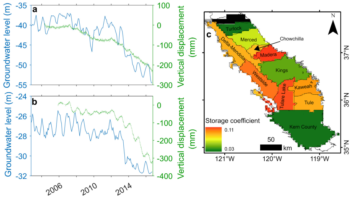
Fig. 7. Computation of inelastic storage coefficient. (a) and (b) shows modeled groundwater level and vertical displacement from GPS at sites P304 and P545 (shown in Fig. 1), respectively. (c) the inelastic storage coefficients for subbasins computed from modeled groundwater level and vertical displacement data from CS-2 altimeter.
