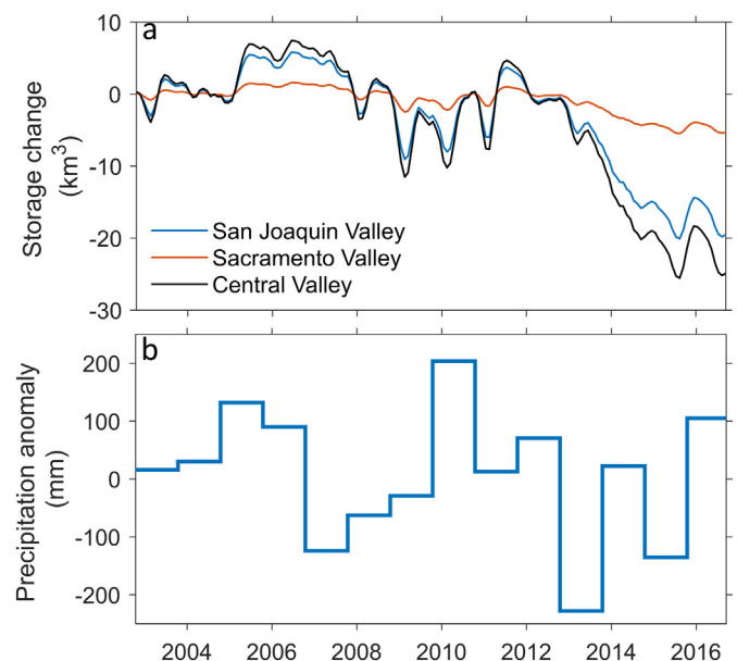
Fig. 8. (a) Temporal variations of groundwater storage in Central, San Joaquin and Sacramento Valley, and (b) annual precipitation anomalies in the Central Valley.
