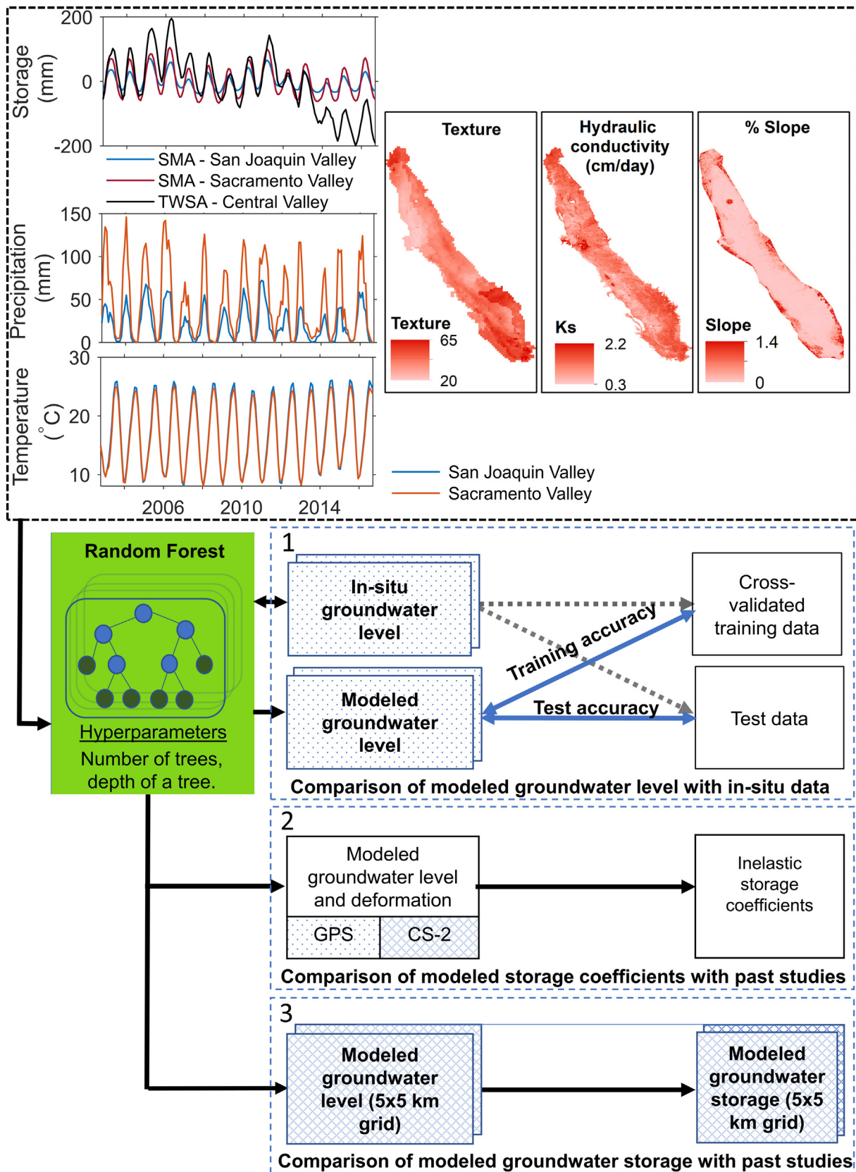
Fig. 2. The workflow used for downscaling GRACE data and modeling groundwater changes using Random Forest.
