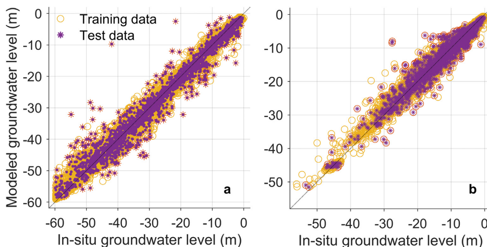
Fig. 4. The accuracy assessment for RF machine learning modeling. Correlation plots between the modeled results and in situ groundwater level variations for training and test data for (a) San Joaquin and (b) Sacramento Valley, respectively.
