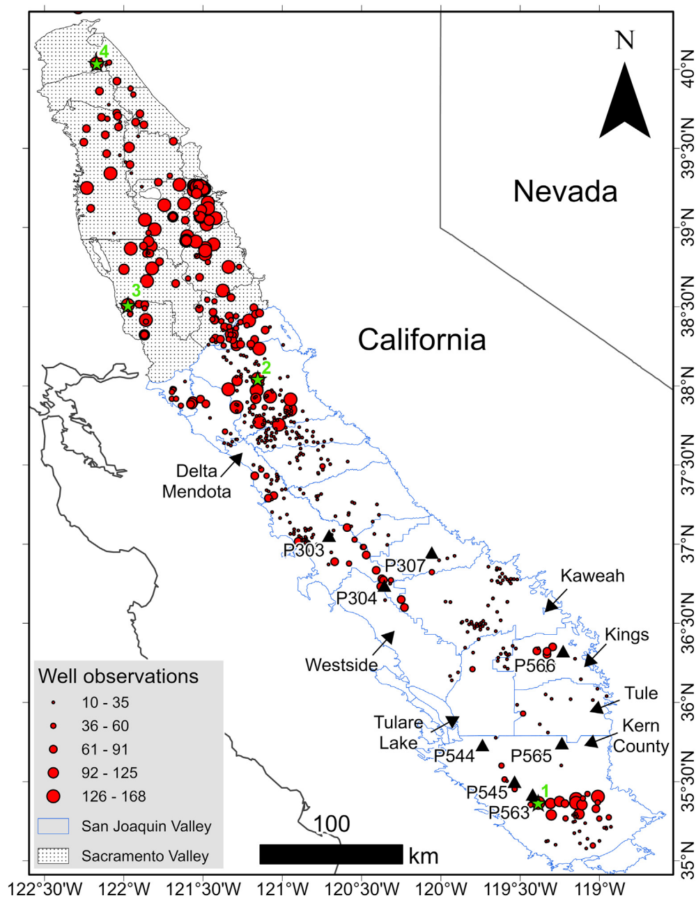
Fig. 1. Location of Central Valley and borderlines of the two major basins, Sacramento (shaded) and San Joaquin (blue) Valley in north and south, respectively. Some of the subbasins in southern San Joaquin Valley are marked in the figure. The location of wells used in this study and the number of measurements over the study period is also shown with solid red circles. 7 GPS sites used in this study are shown by solid black triangles. The green stars represent the wells used for validation studies and for plotting in Fig. 6. (For interpretation of the references to colour in this figure legend, the reader is referred to the web version of this article.)
