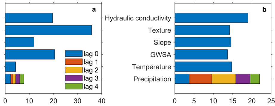
Fig. 5. Feature importance plots based on OOB permutations for (a) San Joaquin and (b) Sacramento Valley.
