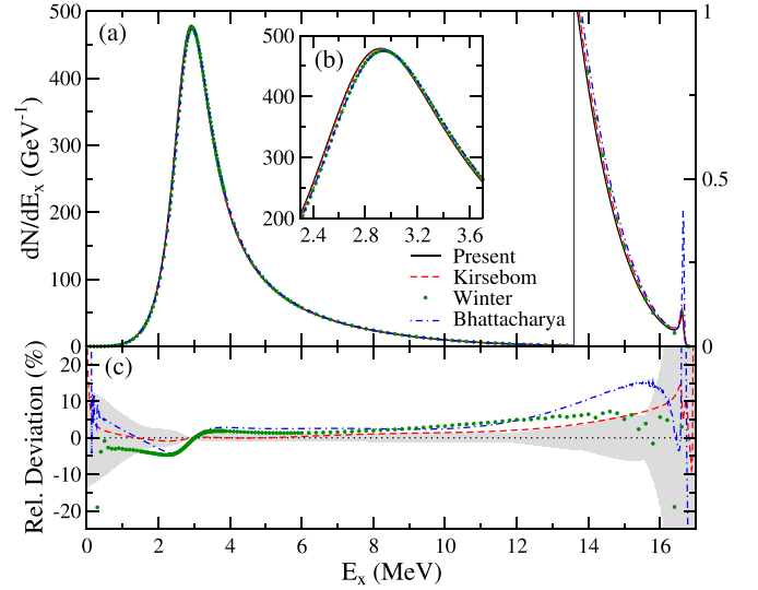
FIG. 2. Panel (a) shows the present FSD (black solid curve) compared to Kirsebom et al. [23] (red dashed curve), Winter et al. [21] (green dots), and Bhattacharya et al. [22] (blue dot-dashed curve). Panel (b) highlights the peak region. Panel (c) shows the relative deviations (\text{FSD} - \text{FSD}_{\text{present}})/\text{FSD}_{\text{present}} . The gray band represents the 1\sigma uncertainty for the present FSD.
