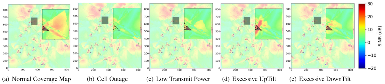
FIGURE 3. REMs presenting different network conditions. (a) Normal, (b) cell outage, (c) low transmission power, this image is showing when transmission power drops to 25dBm, (d) excessive antenna up tilt, this is +20^\circ tilt, and (e) excessive antenna down tilt, -20^\circ tilt.
