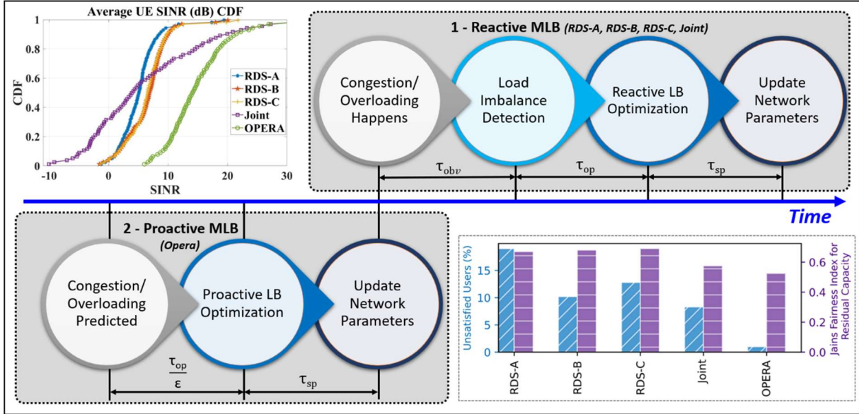
Fig. 4. Gain in QoE achieved by using P-MLB based OPERA framework [12].
