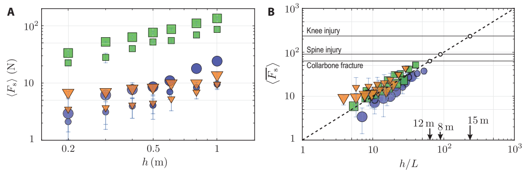
Fig. 5. Variation of the time-averaged impulse with diving height. (A) Time-averaged impulse for hand-first (orange triangles), head-first (blue circles), and feet-first (green squares) impacts for different diving heights. Marker sizes represent data for two separate sizes of each model. (B) Rescaling the effective slamming force and impact height leads to the collapse of the data onto the master curve given by \langle F_s \rangle = h/L , which is represented by the solid dashed line. Critical force values from Table 1 are plotted as the horizontal lines. The open circles represent critical heights for head-first (8 m), hand-first (12 m), and feet-first (15 m) dives causing injury. These dimensional heights correspond to an average body size ( L ) listed in Table 1.
