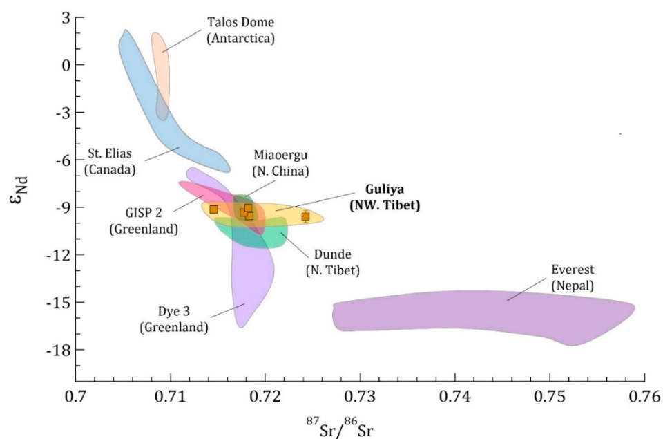
Figure A6. \epsilon_{Nd} vs. ^{87}Sr/^{86}Sr of the five Guliya dust filters (brown squares) compared to Sr and Nd isotopic arrays of dust sampled in ice cores from: Dundee (China [35]), Miaogou (China [43]), Everest (Nepal [44]), Mt. St. Elias (Canada [34]), GISP2 (Greenland [26]), Dye 3 (Greenland [22]) and Talos Dome (Antarctica [100]). These ice cores cover different time scales.
