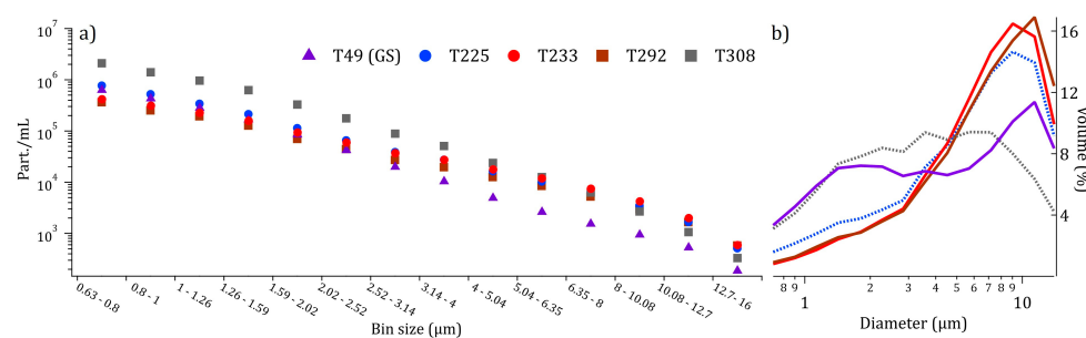
Figure 4. (a) number and (b) relative volumetric size distribution of microparticles measured by Coulter counter (14 bins) in 1 m ice sections prior to filtering.
