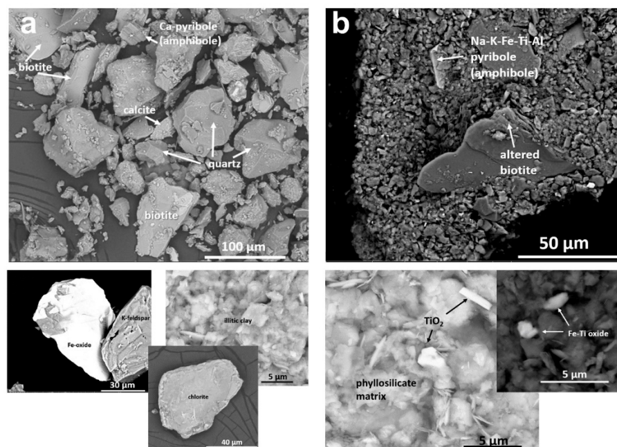
Figure 5. SEM (Scanning Electron Microscope) images of dust filters collected from (a) GS (T50) and (b) GP (T309).
