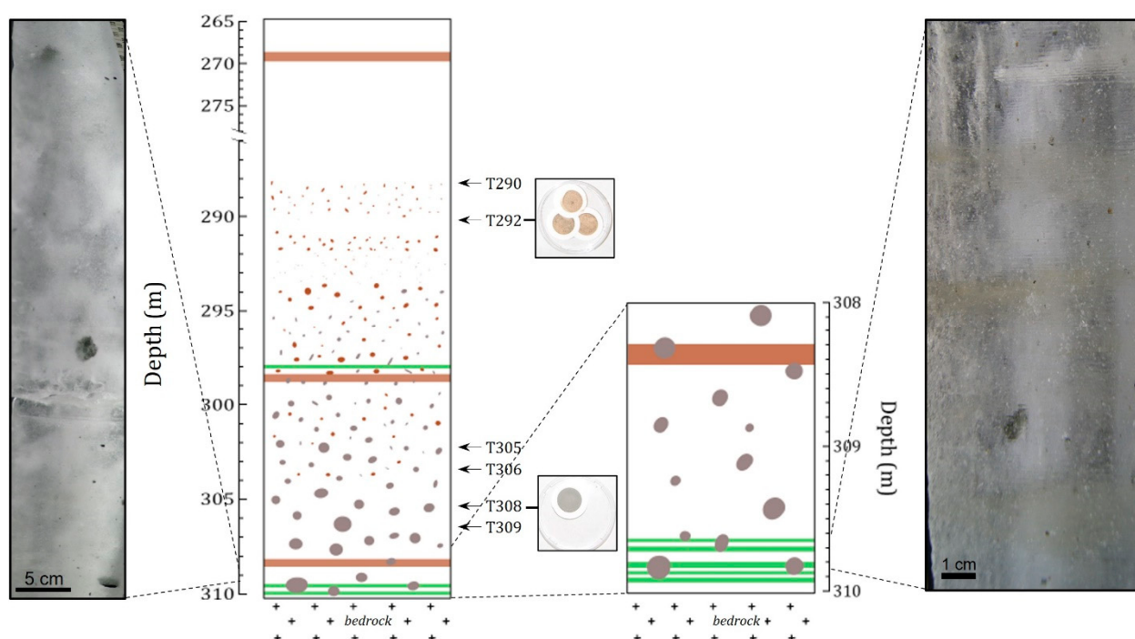
Figure A1. Simplified visual stratigraphy of the deepest 45 m of the GP ice core. Horizontal bars in the sketch mark the location of diffuse brown or greenish dust layers. Dots of various sizes symbolize dust particles and nodules. The grey dust nodules are larger within the deepest 5 m of the core. Note that the size of particles and nodules is not at scale in the sketch. The arrows point to the top depth of the 6 deepest 1 m ice sections discussed in this paper. The color difference is still noticeable among dust filters, as shown here in small photos of T292 and T308 filters. Photos of deep ice core sections show the grey nodules (T311, left) and horizontal diffuse layers (T312, right). Bubbles are present throughout the core and extend all the way to the bedrock, confirming the ice's meteoritic nature. The nodules' increasing size with depth could reflect growth by aggregation with time [60]. Smaller and much less conspicuous grey nodules have been observed in shallower parts of the GP core, which are not discussed in this paper.
