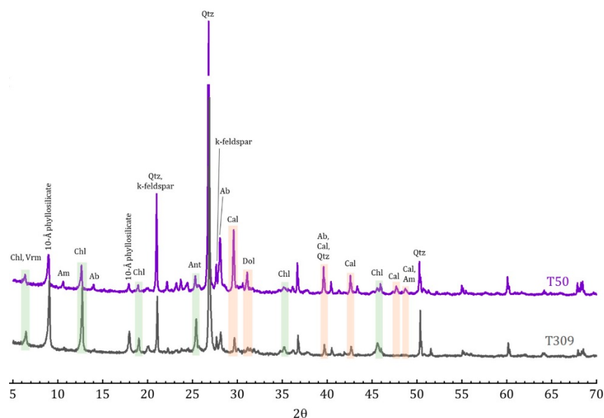
Figure 6. X-ray diffraction (XRD) patterns for the dust sampled from the deepest layers of the GS (T50) and the GP (T309) cores discussed in this study. The T50 diffractogram is shifted up to allow the identification of key features and to facilitate the visual comparison with T309. The orange and green shadings highlight minerals found in higher abundance, respectively, in T50 and in T309 (conventional mineral abbreviations from USGS.gov).
