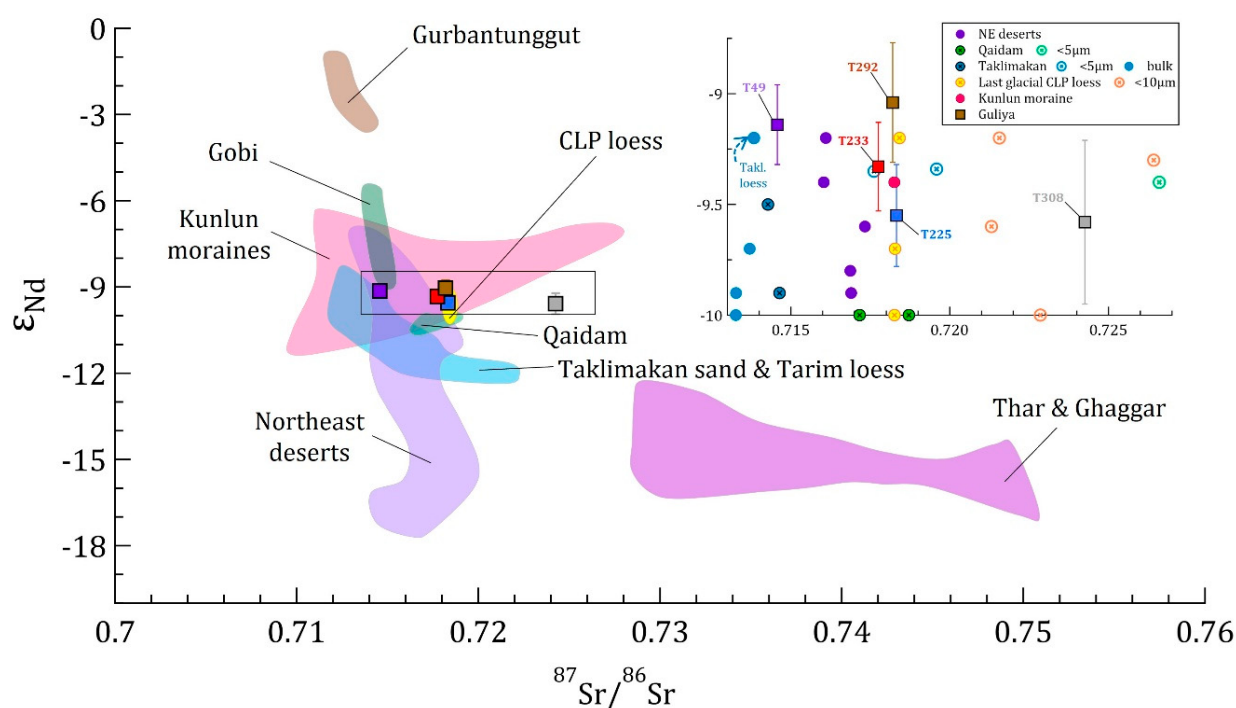
Figure 11. \epsilon_{\text{Nd}} vs. ^{87}\text{Sr}/^{86}\text{Sr} of the five Guliya dust filters (squares) compared to Sr and Nd isotopic arrays of ( <75 \mu\text{m} ) dust sampled in Chinese deserts: Gurbantunggut, Qaidam [37], Gobi [26], Taklimakan sand and Tarim loess [36,37], Kunlun moraines [92], CLP loess [37], Northeast deserts including Mu Us, Hobq and Badain Jaran deserts [36]; and Indian deserts Thar [39] and Ghaggar river sediments [103]. The inset identifies the dust filter samples (squares) shown in the main figure and individual data points for the Chinese deserts' arrays within the rectangle. Data points for the clay-size fraction of surface Qaidam sand ( <5 \mu\text{m} , [37]) and last glacial CLP loess ( <10 \mu\text{m} , [30]) are also shown (crossed circles) as they can be compared to the naturally size sorted T308 sample (fine grey clay).
