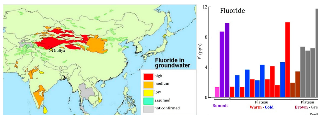
Figure A4. Probability of occurrence of excessive fluoride concentrations in Asian groundwater (left panel) [85] and median fluoride concentration (ppb) measured in 1 m ice samples from the Guliya ice cores discussed in this paper (right panel).
