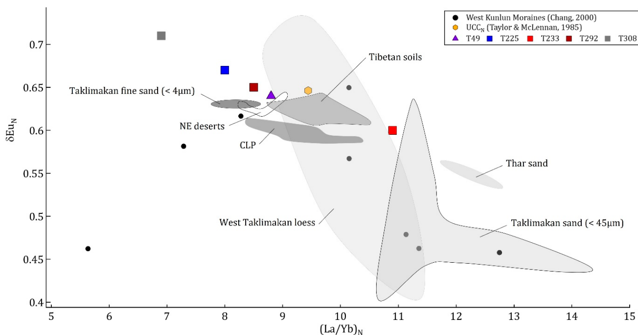
Figure 10. REE-based provenance signatures of Guliya dust filters compared to that of Central Asian dust sources: Chinese Loess Plateau (CLP) loess; Taklimakan fine sand; Northeast deserts (Mu Us, Hobq, and Badain Jaran deserts); Tibetan soils, and Thar desert [76]; West Kunlun moraines [92]; and Taklimakan sand and West Taklimakan loess [36]. The N subscript in \delta\text{Eu}_N and (\text{La}/\text{Yb})_N indicates that values are normalized to the C1 chondrite [94].
