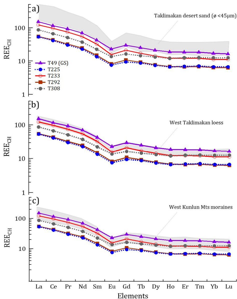
Figure 9. Chondrite-normalized REE patterns of dust filters from GS and GP ice cores compared to Taklimakan fine desert sand, West Taklimakan loess [36] and to moraines of west Kunlun
