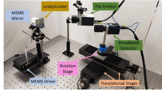
Figure 12: Our experimental setup.
