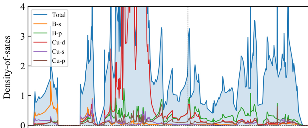
Figure 7. Total and partial density of states of the CuB monolayer.
