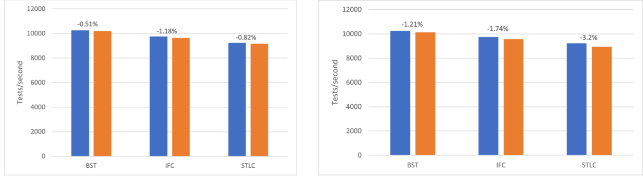
Figure 3. Throughput of QuickChick case studies using handwritten or derived checkers (left) and generators (right).
