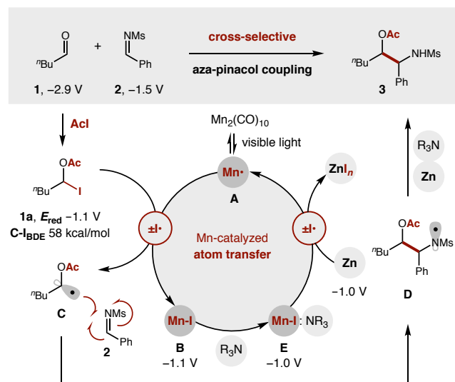
Figure 5. Proposed mechanism of Mn-catalyzed aza-pinacol coupling.
