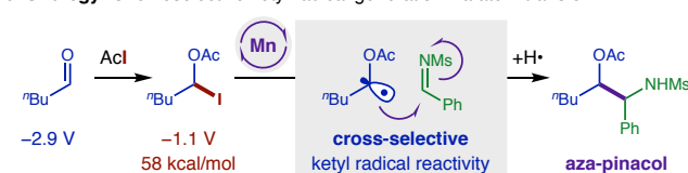
Figure 1. Design of cross-selective strategy for aza-pinacol coupling.
