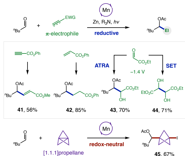
Figure 3. Additional classes of ketyl couplings enabled by atom-transfer catalysis.
