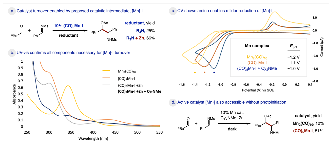
Figure 4. Mechanistic experiments probing Mn catalyst turnover.
