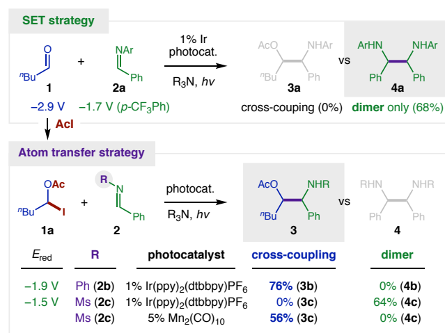
Figure 2. Development of cross-selective aza-pinacol coupling.
