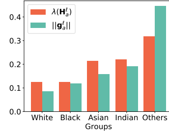
Figure 6: Group Hessians and gradient norms.
