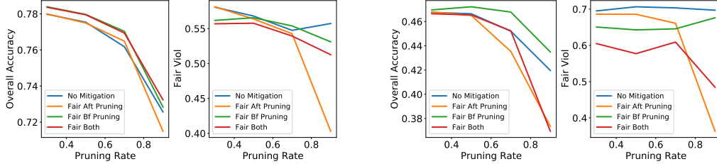
Figure 8: Accuracy and Fairness violations attained by all models on ResNet50, UTK-Face dataset with ethnicity (5 classes) as group attribute (and labels) [left] and age (9 classes) [right].
