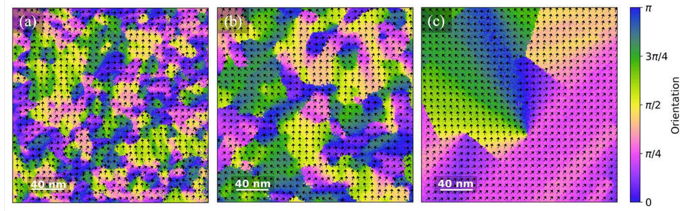
Figure 2. Maps of phenanthroperylene ester column orientation in films deposited at 0.25 Å/s. (a) used a substrate temperature of 380 K ( 0.97 T_g ), and (b) used 392 K ( T_g ). (c) was heated into its liquid crystalline state at 457 K, then cooled to room temperature at 2.5 K/min. The orientation domain size increases with substrate temperature.
