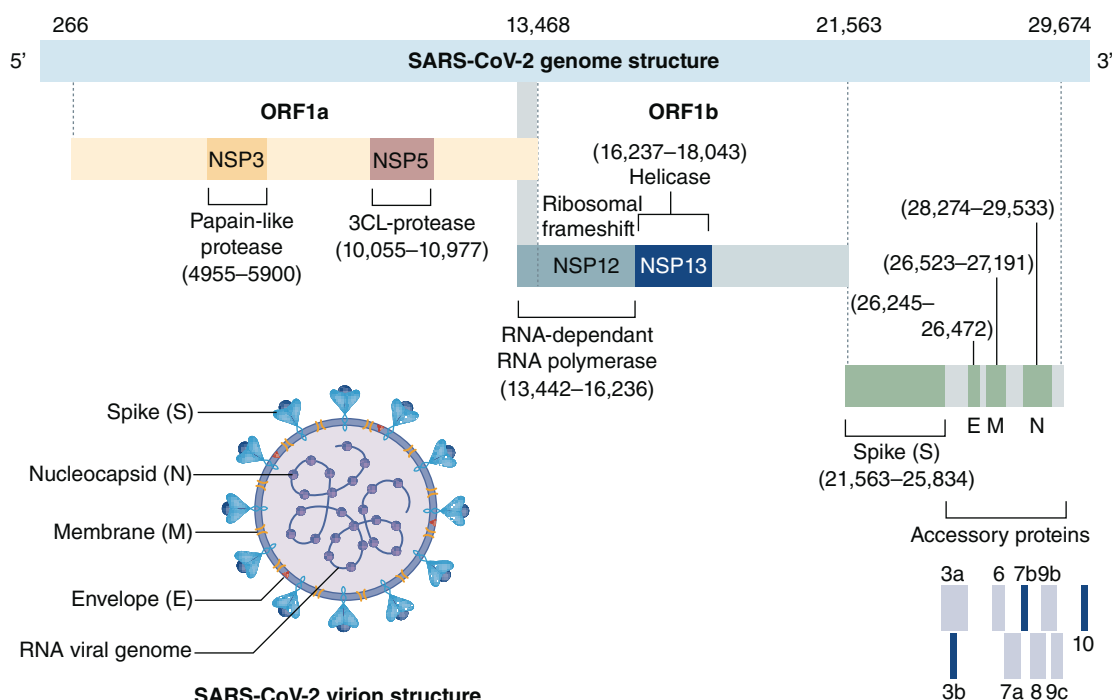
Figure 1. Genomic structure of SARS-CoV-2.
