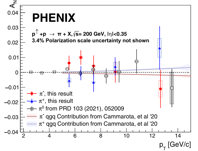
FIG. 3. Transverse-single-spin asymmetries as a function of transverse momentum for positive [closed (blue) triangles], negative [closed (red) circles], and the previously published neutral pions [open (black) boxes]. The statistical uncertainties are shown by bars and the systematic uncertainties are shown by boxes. The lower (red) and upper (blue) curves show the predicted A_N and their uncertainties based on Ref. [16].
