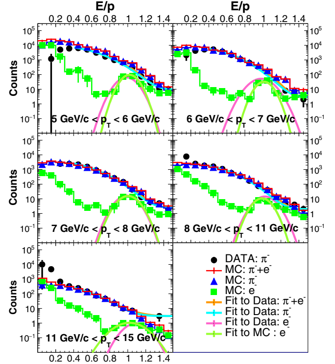
FIG. 2. Energy-over-momentum ratio distribution for negative pion and electron candidates from data and MC simulation for the pion-enhanced data sample.
