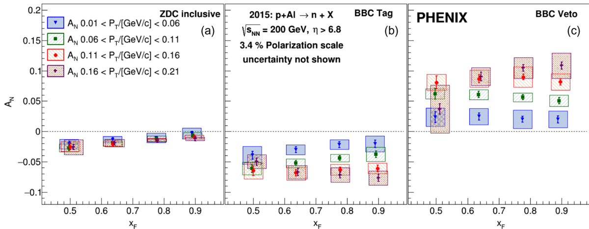
FIG. 7. Single spin asymmetries A_N for very forward neutrons in p + \text{Al} collisions as a function of x_F , in bins of transverse momentum p_T ([blue] triangles, [green] squares, [red] circles, and [purple] crosses in ascending order). The error boxes represent the systematic uncertainties of the asymmetries. The size of the uncertainty boxes does not reflect the bin boundaries and is chosen for visualization purposes. The three panels display (a) inclusive neutron asymmetries, (b) BBC-tagged neutron asymmetries, and (c) BBC-vetoed neutron asymmetries.
