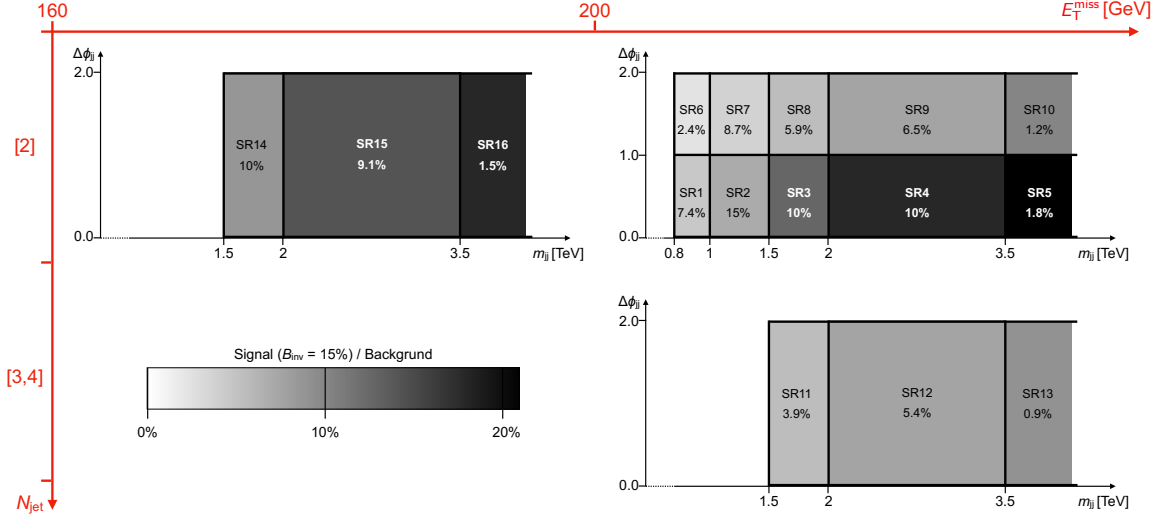
Figure 2. Schematic view of the 16 bins in the signal region. The shading indicates the signal-to-background ratio, assuming a branching fraction of the Higgs boson to invisible particles of B_{inv} = 0.15 . The percentage gives the approximate contribution of signal from invisibly decaying Higgs bosons to each of the bins relative to the total signal yield in the inclusive SR.
