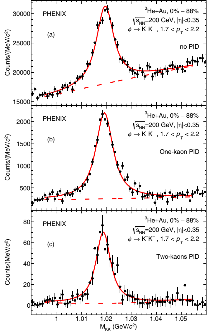
FIG. 1. Examples of invariant-mass distributions for the K^+K^- pairs in {}^3\text{He} + \text{Au} collisions at \sqrt{s_{\text{NN}}} = 200 GeV, obtained with the (a) no PID, (b) one-kaon PID, and (c) two-kaons PID methods after subtraction of the combinatorial background estimated using the event-mixing technique. Plots correspond to integrated p_T for 1.7 < p_T < 2.2 GeV/ c . Spectra are fitted to the sum of a Breit-Wigner function convoluted with a Gaussian to account for the \phi signal, and a polynomial function to account for the residual background.
