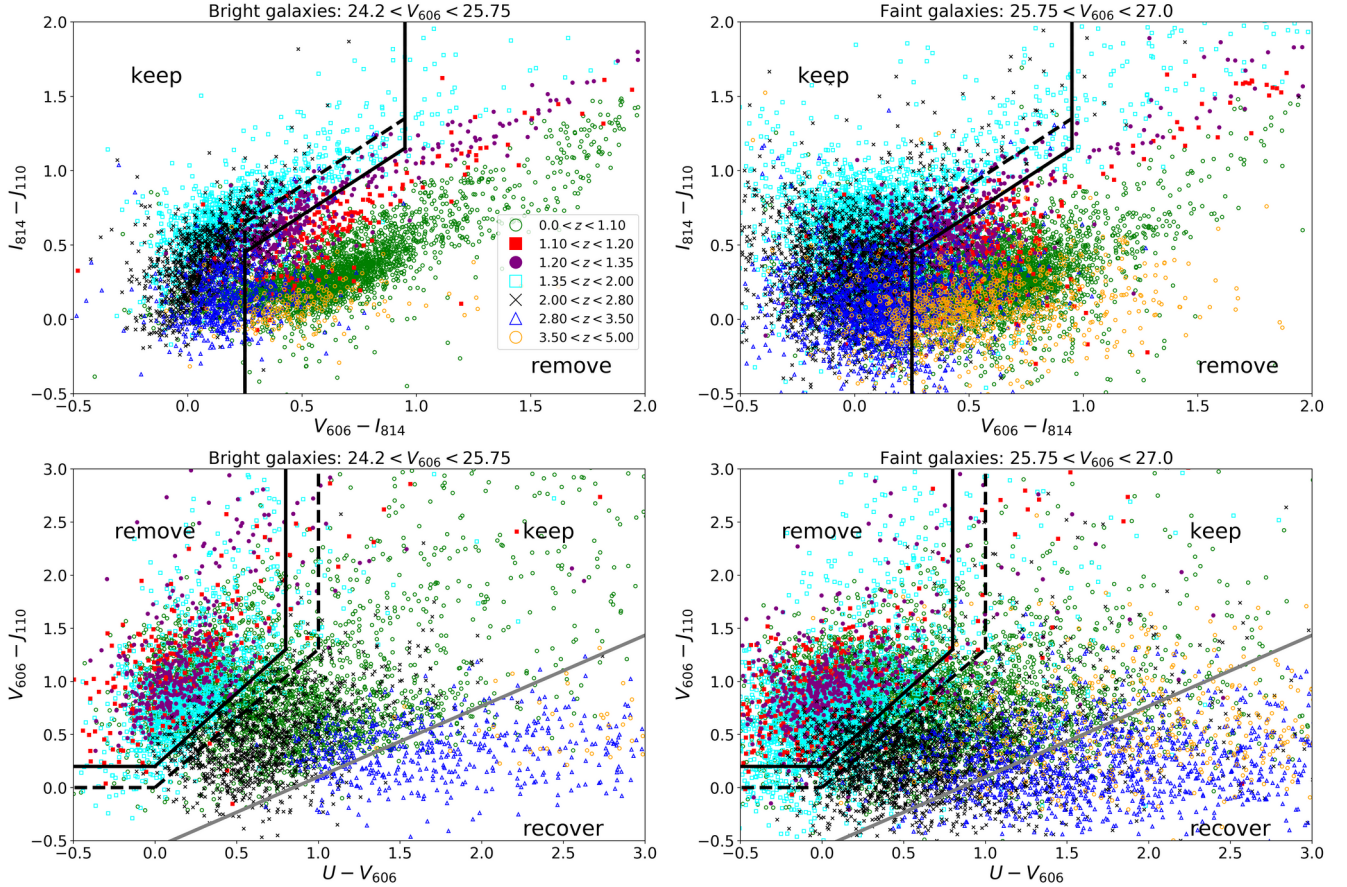
Fig. D.1. First alternative colour selection for galaxy clusters at redshift z \sim 1.2 . The selected source galaxies are at redshift z \sim 1.3 . We display galaxies based on their photometry from S14 in the GOODS-South field. Top: First selection step in the V I J plane for bright galaxies on the left and faint galaxies on the right. Bottom: Second selection step in the U V J plane for bright galaxies on the left and faint galaxies on the right. The solid black lines indicate cuts applied for bright galaxies, the dashed black lines show cuts for faint galaxies. Galaxies below the diagonal grey line are recovered in both the bright and the faint regime.
