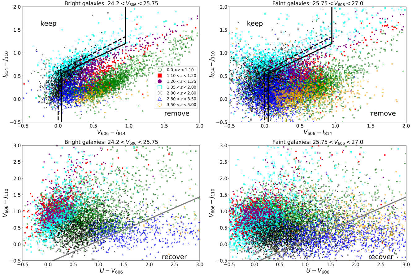
Fig. D.2. Second alternative colour selection for galaxy clusters at redshift z \sim 1.2 . The selected source galaxies are at redshift z \sim 1.3 . We display galaxies based on their photometry from S14 in the GOODS-South field. Top : First selection step in the V I J plane for bright galaxies on the left and faint galaxies on the right. The solid black lines indicate cuts applied for bright galaxies, the dashed black lines show cuts for faint galaxies. Bottom : Second selection step in the U V J plane for bright galaxies on the left and faint galaxies on the right. Galaxies below the diagonal grey line are recovered in both the bright and the faint regime.
