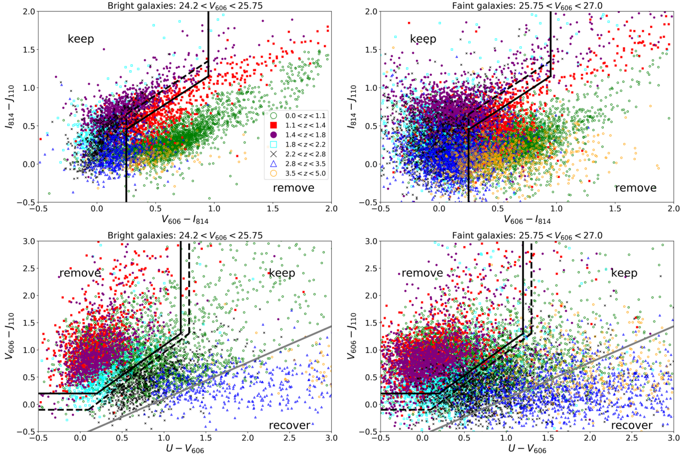
Fig. 3. Colour selection for galaxy clusters at redshift 1.2 < z < 1.7 . The selected source galaxies are at redshift z \approx 1.7 . We display galaxies based on their photometry from S14 in the GOODS-South field. Top : first selection step in the V I J plane for bright galaxies on the left and faint galaxies on the right. Bottom : second selection step in the U V J plane for bright galaxies on the left and faint galaxies on the right. The solid black lines indicate cuts applied for bright galaxies, the dashed black lines show cuts for faint galaxies. Galaxies below the diagonal grey line are recovered in both the bright and the faint regime.
