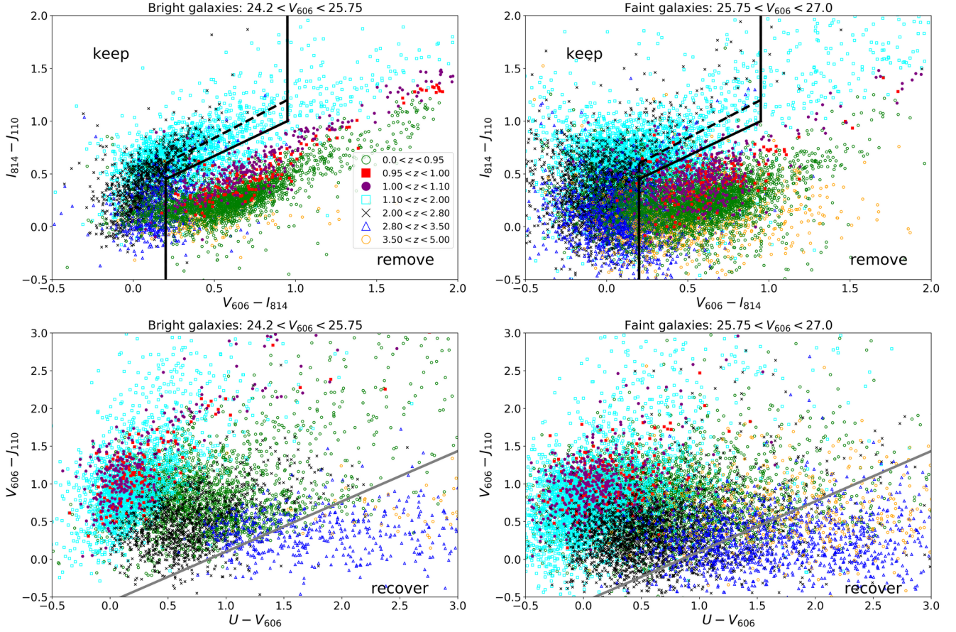
Fig. E.1. Colour selection for galaxy clusters at redshift z \sim 1.0 . The selected source galaxies are at redshift z \gtrsim 1.1 . We display galaxies based on their photometry from S14 in the GOODS-South field. Top : First selection step in the V I J plane for bright galaxies on the left and faint galaxies on the right. The solid black lines indicate cuts applied for bright galaxies, the dashed black lines show cuts for faint galaxies. Bottom : Second selection step in the UVJ plane for bright galaxies on the left and faint galaxies on the right. Galaxies below the diagonal grey line are recovered in both the bright and the faint regime.
