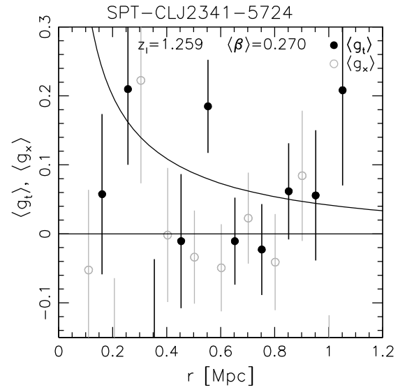
Fig. G.4. Weak lensing results for the clusters in our sample (continued, see the caption of Fig. 9 for details). For SPT-CLJ0646-6236 the reduced shear profile was computed with respect to the SZ centre.
