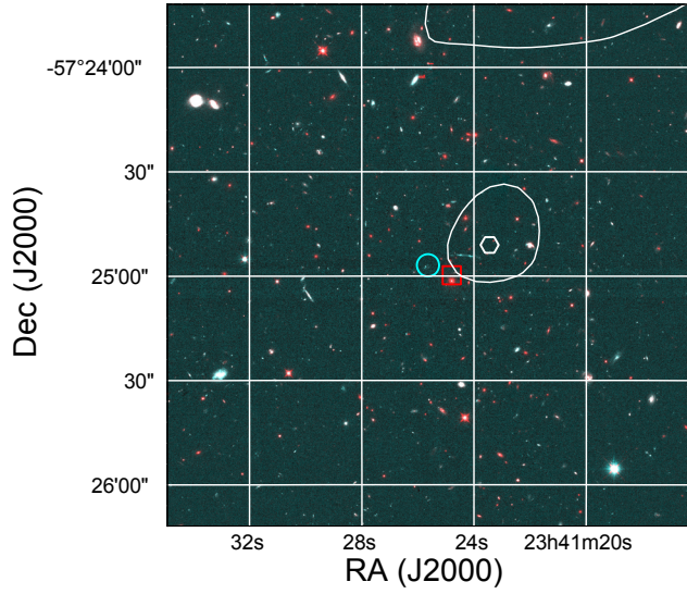
Fig. G.4. Weak lensing results for the clusters in our sample (continued, see the caption of Fig. 9 for details). For SPT-CLJ0646-6236 the reduced shear profile was computed with respect to the SZ centre.
