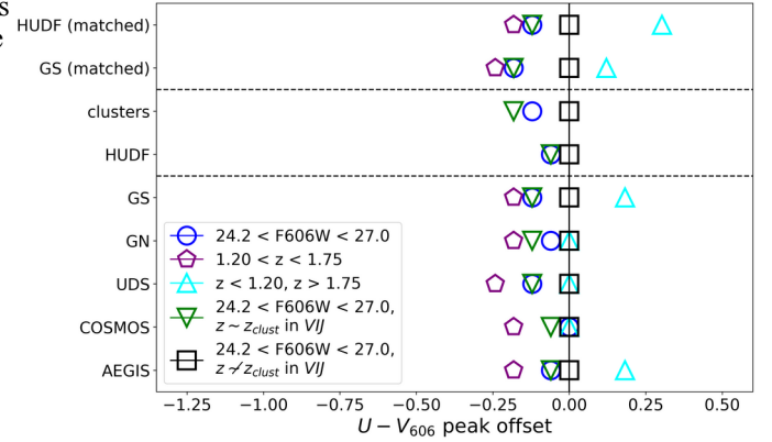
Fig. 2. Offsets between different populations of galaxies and the reference galaxy locus (galaxies with 24.2 < V_{606} < 27.0 , where galaxies at the cluster redshifts 1.2 < z < 1.7 are excluded according to a cut in the VJ colour plane; represented by black squares). Overall the populations exhibit quite similar offsets in U - V_{606} colour despite relying on different U bands. Top section: comparison of directly matched galaxies in the HUDF region based on our measurements and the catalogue in GOODS-South by Skelton et al. (2014). Mid section: comparison of cluster fields (measurements from all nine cluster fields combined) and our measurements in the HUDF area, where we have U_{\text{HIGH}} imaging. Since we do not have photometric redshifts available, the populations relying on these are missing (purple pentagons and cyan triangles). Bottom section: comparisons for five CANDELS/3D-HST fields.
