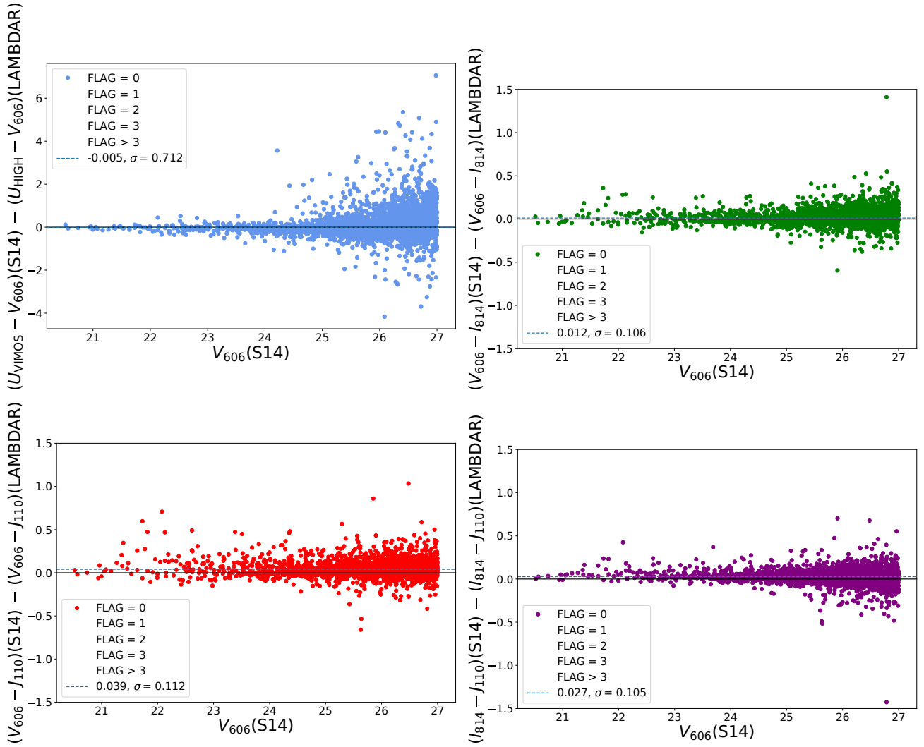
Fig. A.2. Colour differences between S14 and LAMBDAR photometry for the colours U_{\text{HIGH}} - V_{606} , V_{606} - I_{814} , V_{606} - J_{110} , and I_{814} - J_{110} . The blue dashed lines represent the median and we indicate the scatter of the respective colours in the legend label. We show all matched galaxies down to V_{606} < 27.0 mag. We note the different scales on the y-axis for the U - V_{606} colour and the HST -based colours.
