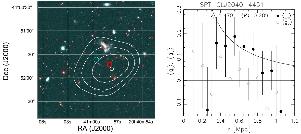
Fig. 9. Weak lensing results for SPT-CL J2040-4451. Left: signal-to-noise ratio contours of the mass reconstruction, starting at \alpha in steps of 0.5\sigma , overlaid on a F606W/F814W/F110W colour image ( 25 \times 25 cutout). The peak in the S/N map is indicated by the hexagon (excluding potential spurious secondary peaks near the edge of the field of view). The cyan circle and the red square show the locations of the SZ peak and the X-ray centroid, respectively. Right: reduced shear profile around the X-ray centre, including the tangential component (solid black circles including the best-fitting NFW model) and the cross component (open grey circles), which has been shifted along the x -axis for clarity. The results for the other clusters are shown in Appendix G.
