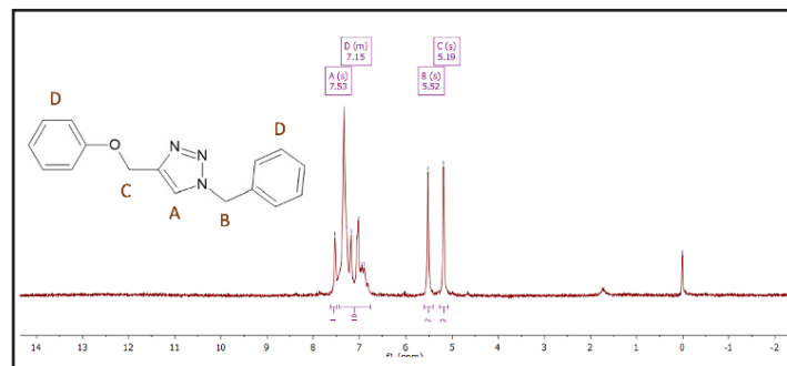
Figure 8. ^1\text{H} NMR spectrum for 1-benzyl-4-(phenoxy)methyl-1H-1,2,3-triazole (product 1 ).
