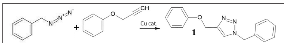
Scheme 2. Cu-catalyzed click reaction of benzyl azide and phenyl propargyl ether to produce 1-benzyl-4-(benzyloxy)-1H-1,2,3-triazole (product 1).
