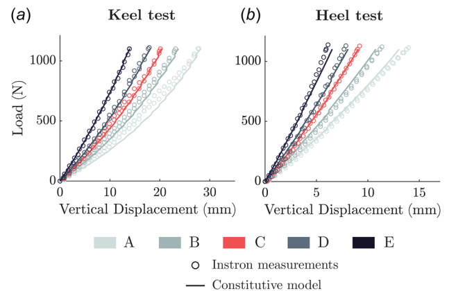
Fig. 6 Load-displacement curves of participant 4's foot conditions (A-E) measured with the Instron machine and compared to the constitutive model. (a) Keel loading tests at CoP_{Keel} = 130 \pm 0.1 mm. (b) Heel loading tests with CoP_{heel} = -30 \pm 0.1 mm. Load displacement results for other participants are shown in Appendix A.
