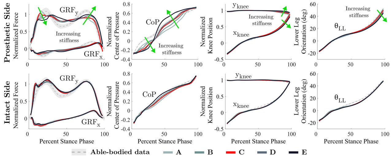
Fig. 16 Average kinetic and kinematic variables over the entire stance phase for participant 5 for each prosthetic foot type averaged across steps. This includes horizontal and vertical ground reaction forces ( GRF_x and GRF_y ), center of pressure (CoP) progression, and lower leg position and orientation in the sagittal plane ( x_{knee} , y_{knee} , and \theta_{LL} ) for both the prosthetic and intact side. The shaded regions correspond to one standard deviation of the normative physiological data.
