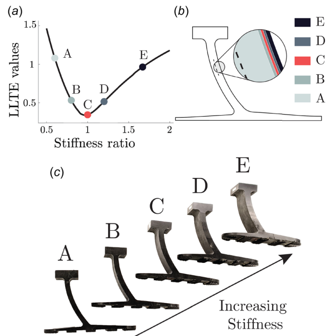
Fig. 3 Prosthetic foot prototypes labeled A-E used by participant 3 in the gait study, with A corresponding to the most compliant, E the stiffest, and C the predicted LLTE-optimized foot: (a) LLTE values and stiffness ratio for each prosthetic foot condition, (b) beam thickness variation that resulted in the stiffness change for each foot prototype. The dashed line represents the beam section neutral axis, and (c) photographs of the manufactured prototype feet.
