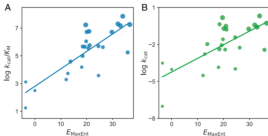
Fig. 2. The maximum entropy model for natural sequences is correlated with the catalytic power of designs in directed evolution. Strong positive correlations between E_{\text{MaxEnt}} and \log k_{\text{cat}}/K_M (A) and \log k_{\text{cat}} (B) for the KE07-directed evolution are shown with the least-squares regression lines included. Each dot represents a design with a larger dot size indicating later rounds in directed evolution. We shifted E_{\text{MaxEnt}} by a constant so that the initial design has a zero value.
