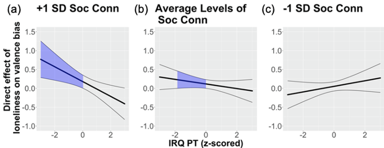
Fig. 2. Regions of significance for the relationship between loneliness and a more negative valence bias at each level of IER for (a) +1 SD, (b) mean, and (c) –1 SD social connectedness.
