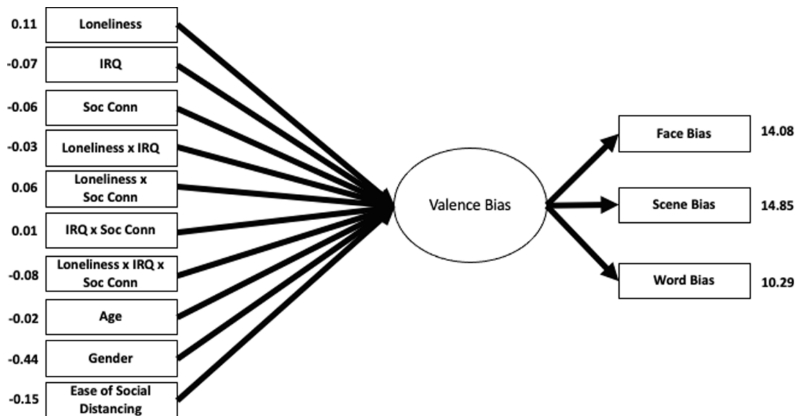
Fig. 1. Path Diagram of Structural Equation Model. Note: Factor loadings are shown for the indicators of valence bias and unstandardized estimates are shown for exogenous variables. Intercept and residual estimates are not shown. Soc Conn = Social Connectedness, Gender (0 = Female, 1 = Male).
