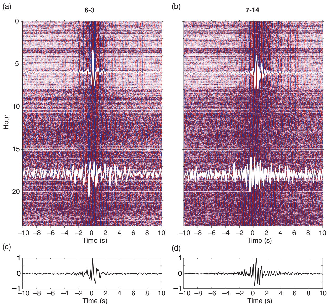
Figure 4. (a) Temporal variation of 5-min cross-correlations functions (CCFs) of station pair 6–3 on 7/26. Positive and negative CCF amplitudes are shaded in different tones to highlight the coherency through time. The white waveforms are the 5-min CCFs at 6:00 and 18:00. (b) Same as panel (a) but for station pair 7–14, (c) 7/26 daily CCF stack of station pair 6–3, and (d) 7/26 daily CCF stack of station pair 7–14. The color version of this figure is available only in the electronic edition.
