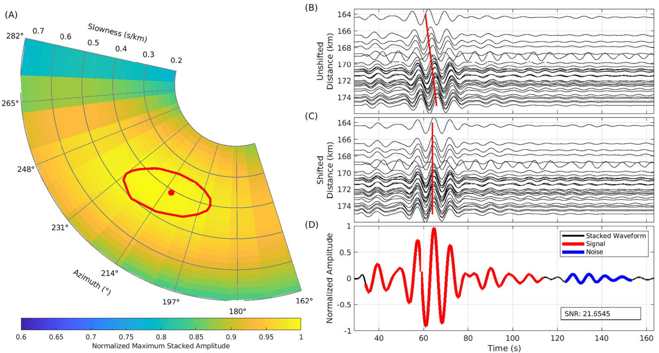
Figure 4. Example beamforming process for one beam center with seismometer VRUT (Figure 1) as the source. This particular beam is in the densest part of the Dog Valley sub-array, resulting in the inclusion of many individual correlograms. Location is shown as a green triangle in Figure 2. (a) Polar plot showing stacked beam amplitude as a function of azimuth and slowness. The maximum amplitude slowness and azimuth is shown as a red dot. 95% of the maximum is contoured in red. (b) Original, un-shifted waveforms. (c) Shifted waveforms corresponding with the maximum stacked amplitude. (d) Stacked waveforms from panel (c), showing the signal and noise windows for SNR calculation. Panels (b–d) share the same time axis.
