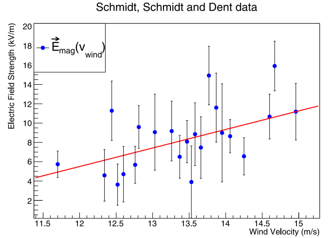
Fig. 2. Electric Field strength vs. wind velocity (data taken from Schmidt, Schmidt and Dent [33]). Overlaid is a linear fit (red line) used to determine the threshold wind velocity.
