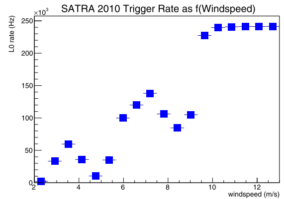
Fig. 18. 2010 SATRA experimental L0 trigger rate dependence on local wind velocity. We observe saturation of the trigger rate at wind velocities above 10 m/s.
