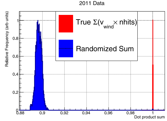
Fig. 10. RICE experiment product of summed values of wind velocity time profile ( v_{\text{wind}}(\text{time}) ) \times average number of hit receiver channels ( N_{\text{hitRx}}(\text{time}) ), for randomized time series of N_{\text{hitRx}} (blue histogram) compared with measured series (red), for 2011. In this Figure, the maximum possible dot product sum has been normalized to 1 on the x-axis.
