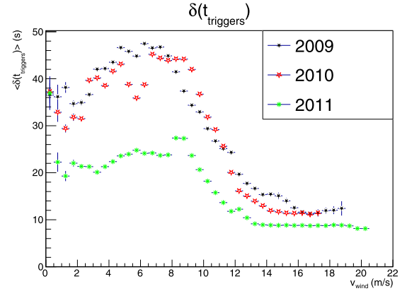
Fig. 12. RICE mean time interval between successive triggers (in units of seconds) as a function of local wind velocity (m/s). The minimum time difference (set by the minimum DAQ reset time) is approximately 0.75 s per active channel. The absolute trigger rate depends on experimental settings and thus varies from year to year. In RICE data, we note amplitude saturation of the data acquisition system throughput at high wind velocities (as also noted below for the SATRA experiment).
