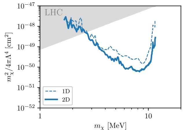
FIG. 5. Limit on the absorption cross section of fermionic dark matter by ^{136}\text{Xe} nuclei at the 90% C.L. We show our main 2D fit result in addition to a deexcitation \gamma agnostic 1D fit result (see text for more details). The gray region is excluded by direct constraint from searches at the LHC [33].
