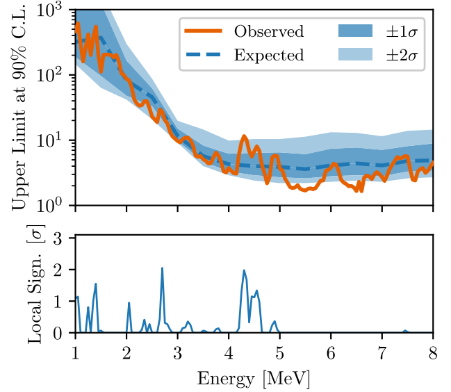
FIG. 4. The top panel of the plot shows the upper limit (solid orange) on the number of dark matter events as a function of the energy at 90% C.L. The median sensitivity (dashed blue) and the \pm 1\sigma (dark blue) and \pm 2\sigma (light blue) percentiles around the median are also shown. The bottom panel shows the local significance of our observation against the no-signal hypothesis.
