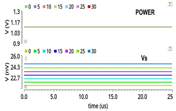
(a) Without modulation at supply line
