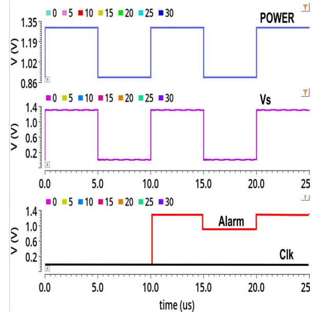
(b) With modulation at supply line
