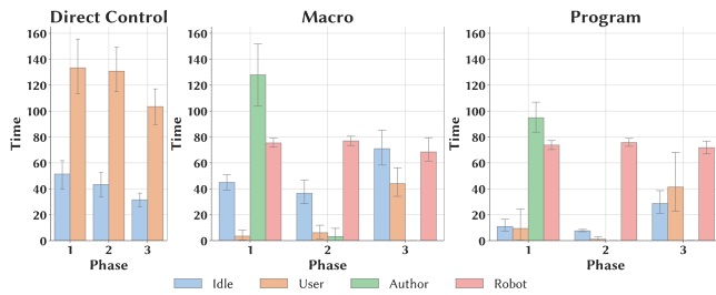
Figure 6: Breakdown of time spent by participants in each technique condition per phase of the evaluation task: (1) Robot idling (waiting for user input). (2) Participant operating the robot. (3) Participant authoring macros and programs. (4) Robot planning and executing trajectories.
