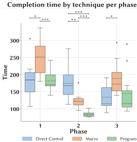
Figure 5: Evaluation task completion times by condition for each phase. Dashed lines represent the mean and the solid lines represent the median. Asterisks indicate pairwise comparisons with significance differences ( p < .05^* , p < .01^{**} , p < .001^{***} ).
