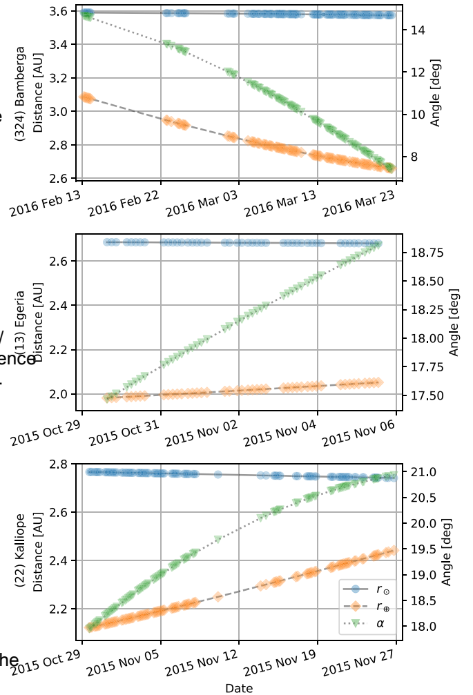
Figure 9. Observation geometries for (324) Bamberga (top panel), (13) Egeria (middle panel), and (22) Kalliope (bottom panel). Each point represents one observation. Solar distance and Earth distance are plotted in astronomical units, and solar phase angle \alpha is plotted in degrees.
