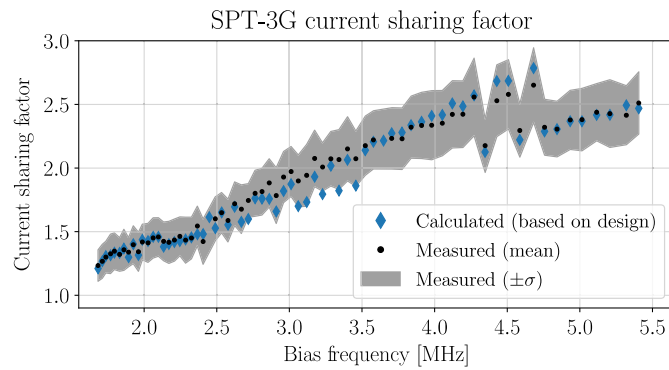
Fig. 13 The current sharing factor \delta I_{cs}/I can be measured directly in situ and compared to an expectation based on an analytic evaluation of the electrical model shown in Fig. 3, which includes both current sharing paths. The plot aforementioned compares the distribution of measured values for each detector across SPT-3G (mean and standard deviation, binned by resonator on the multiplexing module) with a fully analytic expectation based on the readout circuit design. The circuit simulation assumes designed values for all parameters, while the hardware in the receiver includes scatter in detector and filter properties, so width in the measured distribution is expected. The agreement between the simulations and measured values is excellent, and the largest disagreement (between 3 and 3.5 MHz) corresponds to a known region of high scatter in the fabricated LC resonant frequencies, such that neighboring channels are more likely to deviate from the circuit model and have overlapping filters 6 . This suggests that an analytic model for the readout is accurately capturing the relevant dynamics for current sharing effects.
