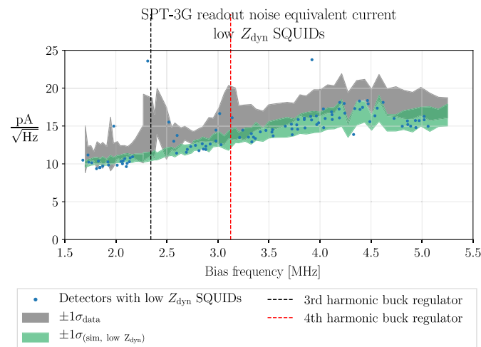
Fig. 11 Measured readout noise in detectors operated with SQUIDs exhibiting a lower dynamic impedance (blue points above) is systematically lower than the rest of the receiver (shown in gray as in Fig. 8). This difference is consistent with the expectation from the noise model, which predicts a \sim 10\% noise improvement at high frequency from lower dynamic impedance SQUIDs. This model is shown in green, where low Z_{\text{dyn}} operation of the entire receiver is simulated. There are currently six SQUIDs on SPT-3G operated at low Z_{\text{dyn}} .
