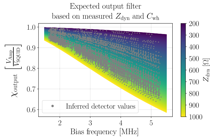
Fig. 10 An analytic calculation of the output filter ( \chi_{\text{output}} ) as a function of SQUID dynamic impedance ( Z_{\text{dyn}} ) for the measured value of C_{\text{wh}} \approx 40 pF. Gray points indicate inferred values for each detector in the receiver, showing that although some detectors benefit from low dynamic impedance SQUIDs, most detectors are significantly attenuated by this filter, especially at high bias frequency. Noise sources in the output signal path are referred to an NEI at the SQUID input by dividing by \chi_{\text{output}} , and therefore appear amplified by this filter.
