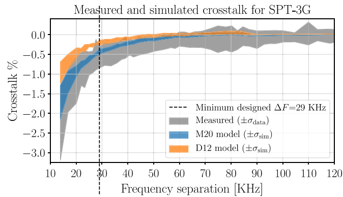
Fig. 7 A comparison between measured in situ crosstalk and simulated crosstalk for 4400 detector pairs in the receiver. Each pair differs slightly in i_{q,r} , R_{TES} , and underlying bias frequencies, all of which are measured separately and used to calculate the total expected crosstalk according to the M20 and D12 analytic models. These results, along with the measured crosstalk values for each detector pair, are shown binned by frequency separation with 1\sigma of distribution in each bin. The M20 model (blue), which includes stray impedances, is a better approximation for the measured crosstalk (gray) than the D12 model (orange), which omits stray impedances. The larger width in the distribution of measured crosstalk reflects the additional scatter associated with fitting noisy optical crosstalk measurements constructed from single-detector maps and template-fitting of an extended source.
