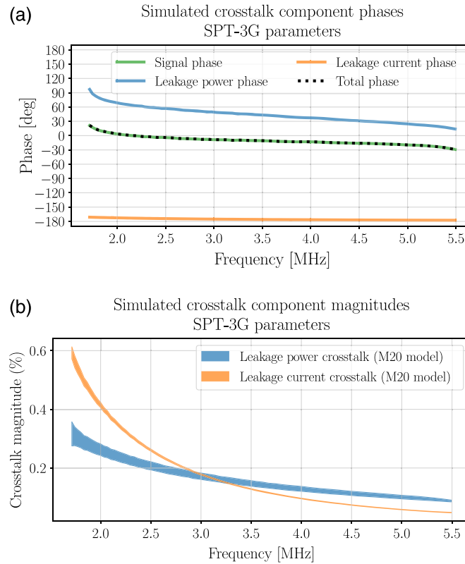
Fig. 5 (a) The phase of each crosstalk component for a simulated SPT-3G multiplexing module with typical properties. The phases \delta_{l,\text{signal}} and \delta_l are nearly identical because the total crosstalk fraction is very low. Most striking, the relative phase offset between the leakage power and the primary signal ranges from between \sim 90 deg and 45 deg, suppressing the effective contribution of leakage power crosstalk. (b) The magnitudes of each crosstalk component for an SPT-3G-like system. Line widths indicate the difference between (i; i \pm 1) and (i; i \mp 1) nearest-neighbor pairs. As magnitudes, both crosstalk quantities are shown as positive; but the relevant quantity is the vector-sum of both crosstalk vectors that is in-phase with the signal. Because leakage current crosstalk is \sim 180 deg out-of-phase with the signal phase it appears as a negative crosstalk. Leakage power crosstalk is, for the most part, < 90 deg out-of-phase with the signal and appears as positive crosstalk. These two end up partially canceling.
