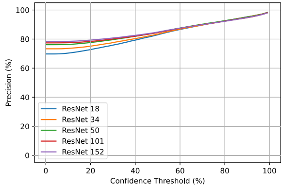
Fig. 2 Populating the model: Setting the confidence threshold
